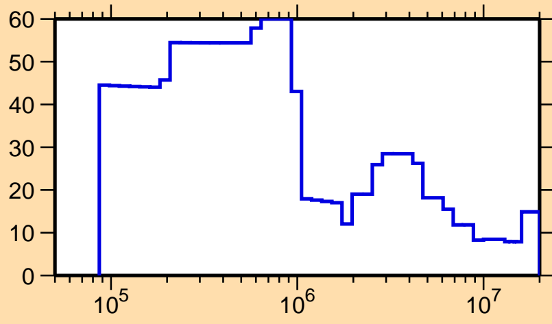
\Delta\sigma/\sigma vs. E for ^{214}\text{Ac}(n,\text{tot.})
