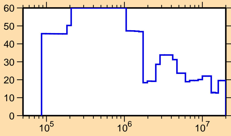
\Delta\sigma/\sigma vs. E for ^{214}\text{Ac}(n,\text{el.})
