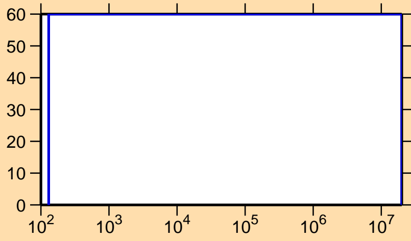
\Delta\sigma/\sigma vs. E for ^{214}\text{Ac}(n,p)
