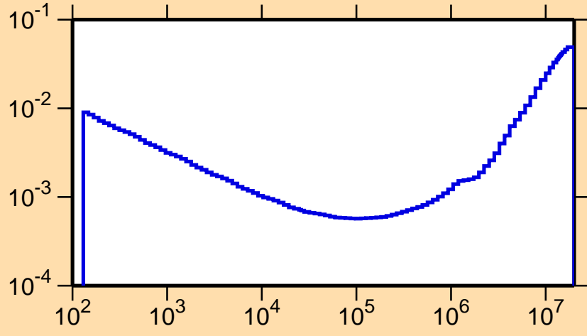
\sigma vs. E for ^{214}\text{Ac}(n,p)
