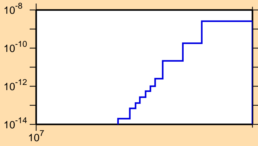
\sigma vs. E for ^{214}\text{Ac} (mt 34)
