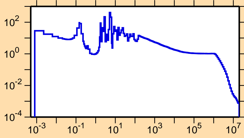
\sigma vs. E for ^{214}\text{Ac}(n,\gamma)
