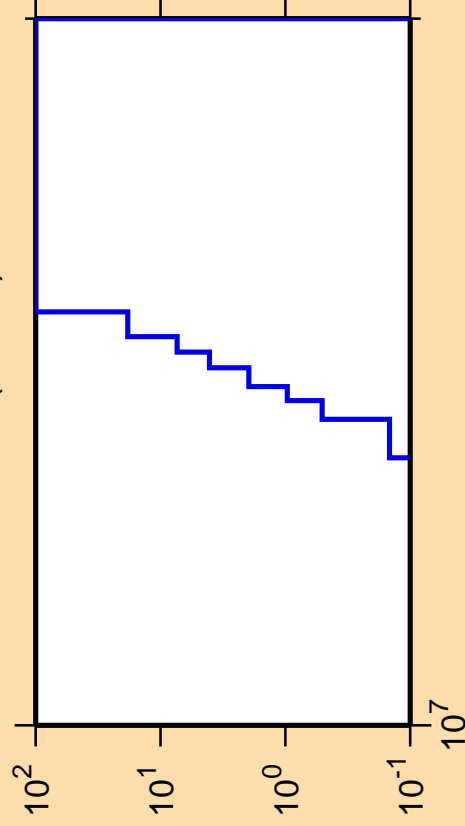
\Delta\sigma/\sigma vs. E for ^{214}\text{Ac} (mt 34)
