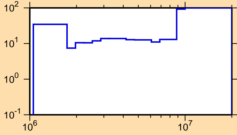
\Delta\sigma/\sigma vs. E for ^{214}\text{Ac}(n,n\text{cont.})
