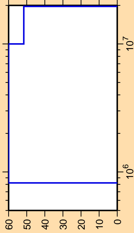
\Delta\sigma/\sigma vs. E for ^{214}\text{Ac}(n,n\alpha)
