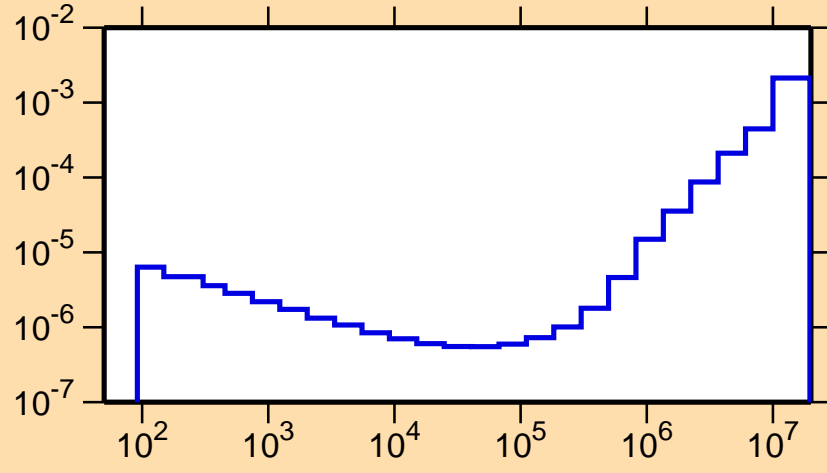
\sigma vs. E for ^{214}\text{Ac}(n,p\alpha)
