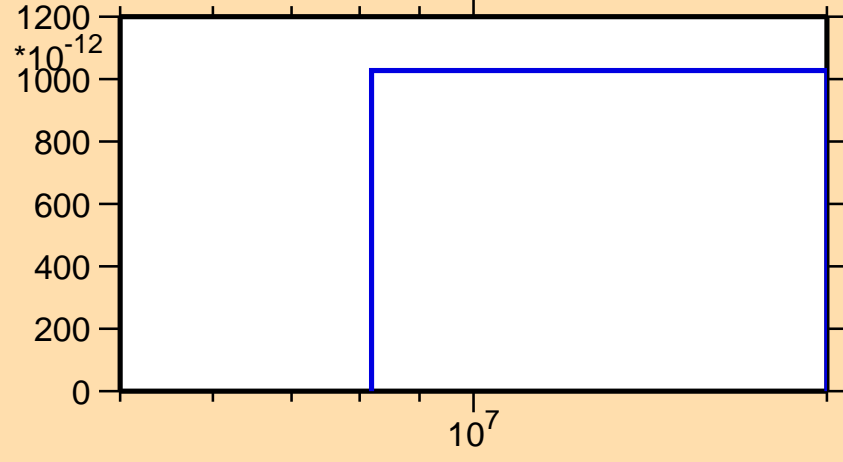
\sigma vs. E for ^{214}\text{Ac}(n,pd)
