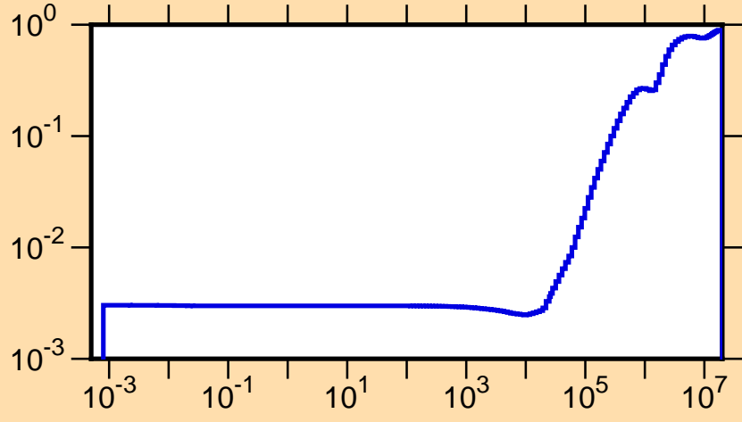
\mu vs. E for ^{222}\text{Ac}(\text{mt251})
