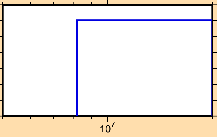
\sigma vs. E for ^{222}\text{Ac}(n,nt)
