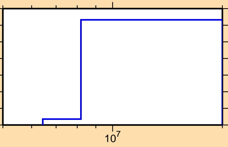
\sigma vs. E for ^{222}\text{Ac}(\text{mt117})
