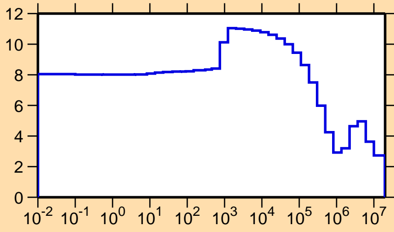
\sigma vs. E for ^{222}\text{Ac}(n,\text{el.})
