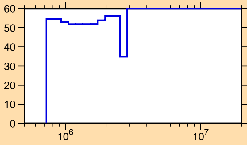
\Delta\sigma/\sigma vs. E for ^{223}\text{Ac}(n,n_1)
