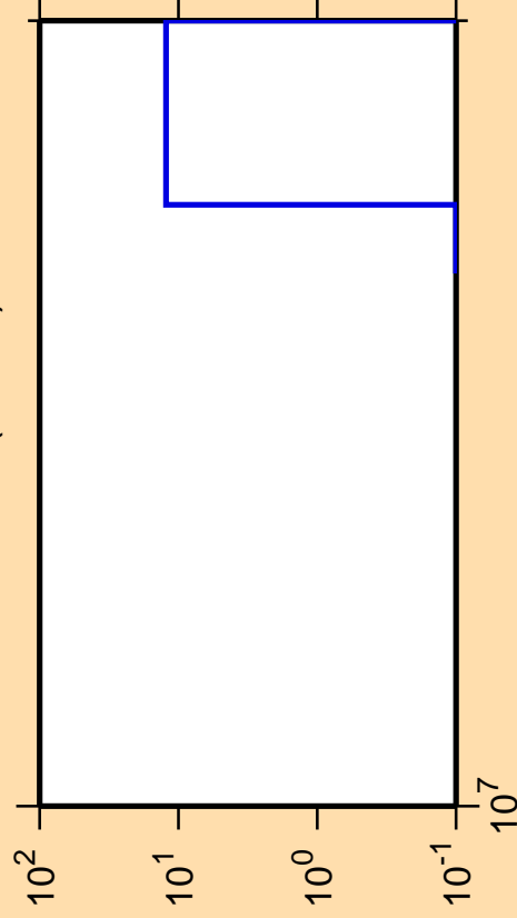
\Delta\sigma/\sigma vs. E for ^{223}\text{Ac} (mt 42)
