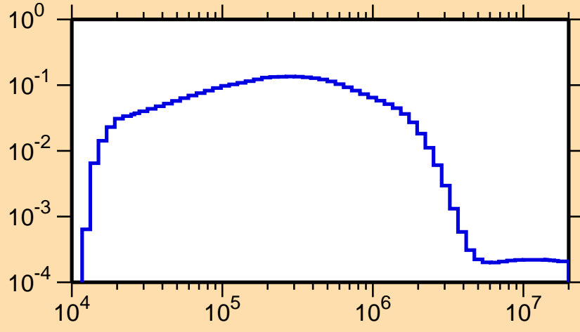
\sigma vs. E for ^{223}\text{Ac}(n,n_1)
