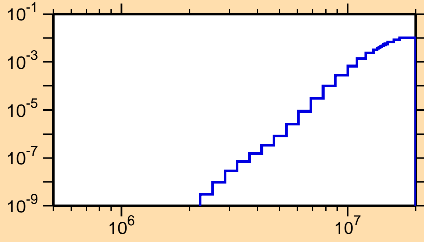
\sigma vs. E for ^{223}\text{Ac}(n,p)
