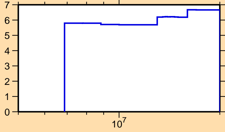
\Delta\sigma/\sigma vs. E for ^{223}\text{Ac}(n,\text{nonel.})
