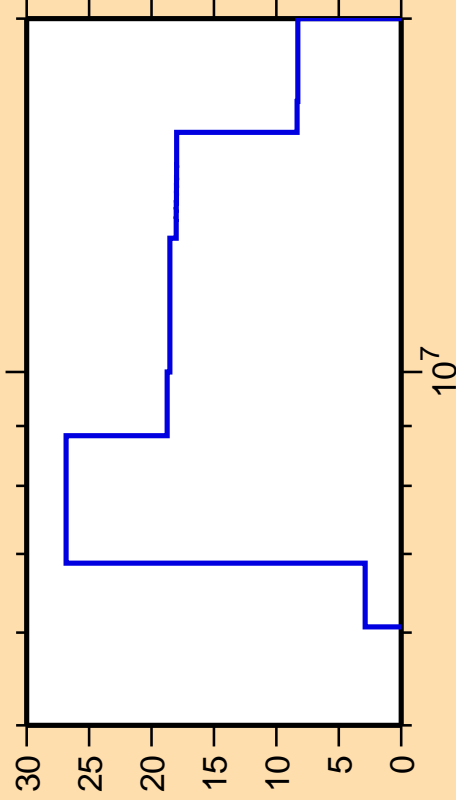
\Delta\sigma/\sigma vs. E for ^{223}\text{Ac}(n,d)
