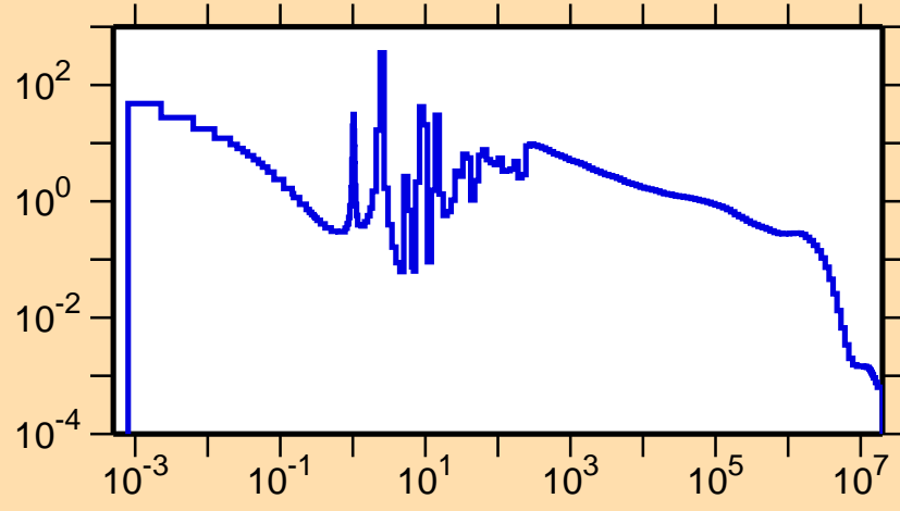
\sigma vs. E for ^{223}\text{Ac}(n,\gamma)
