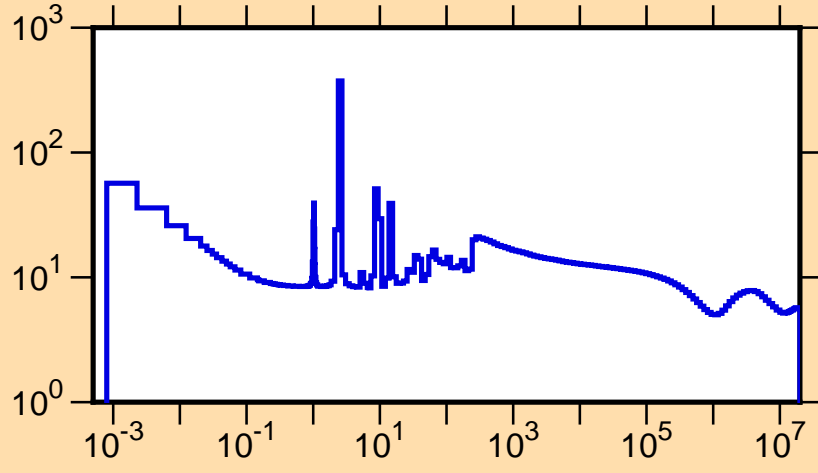
\sigma vs. E for ^{223}\text{Ac}(n,\text{tot.})
