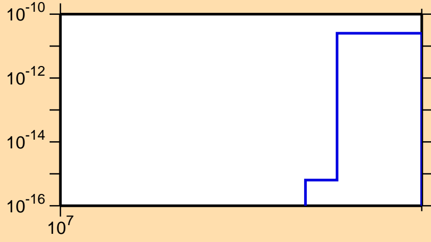
\sigma vs. E for ^{223}\text{Ac} (mt 11)
