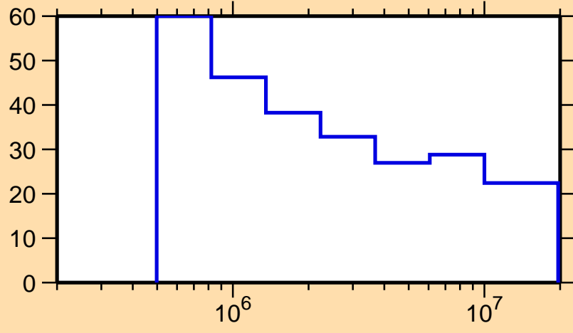
\Delta\sigma/\sigma vs. E for ^{223}\text{Ac}(n,n\text{cont.})
