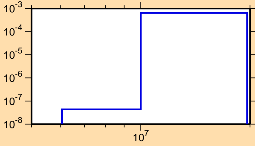
\sigma vs. E for ^{223}\text{Ac}(n,d)
