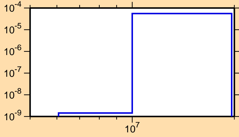
\sigma vs. E for ^{223}\text{Ac}(\text{mt117})
