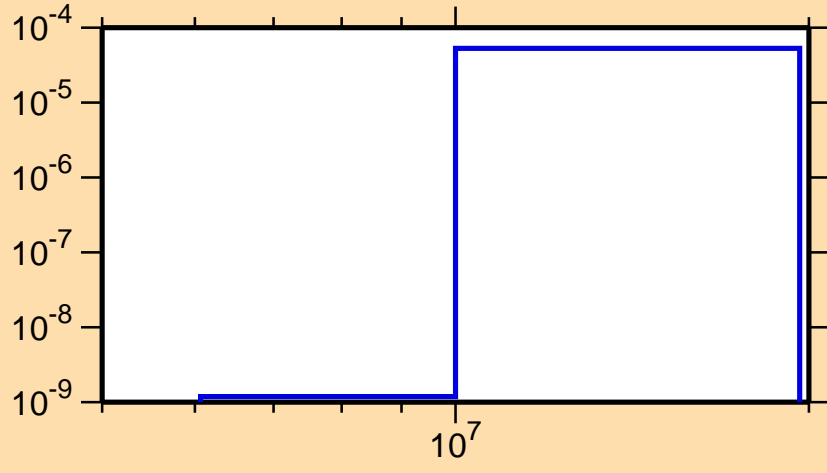
\sigma vs. E for ^{223}\text{Ac}(\text{mt } 45)
