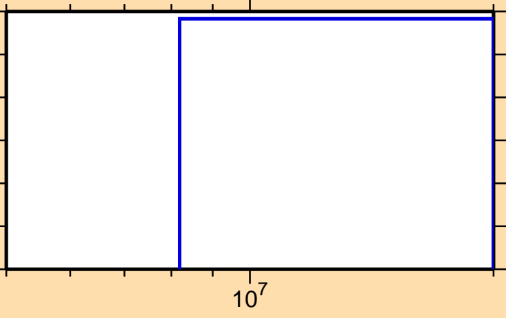
\sigma vs. E for ^{223}\text{Ac}(n,\text{nd})
