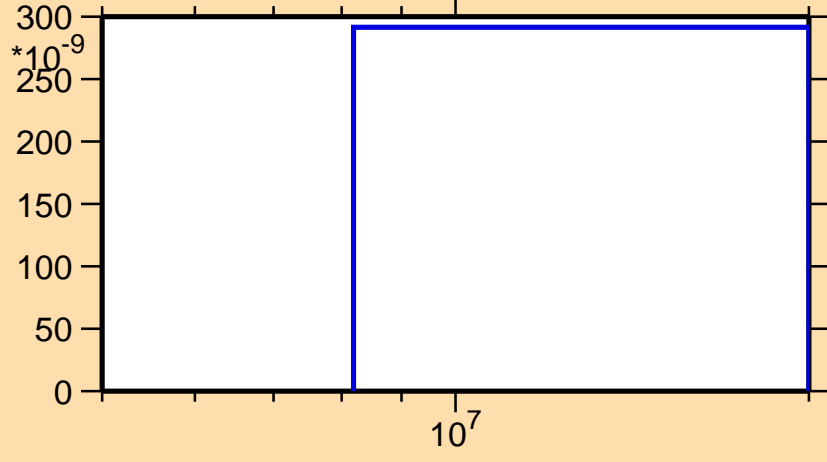
\sigma vs. E for ^{223}\text{Ac}(n,\text{nd})
