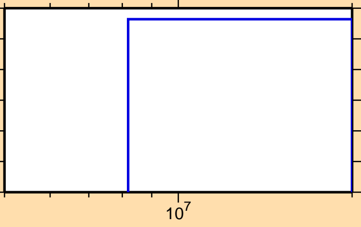
\sigma vs. E for ^{223}\text{Ac}(n,nt)
