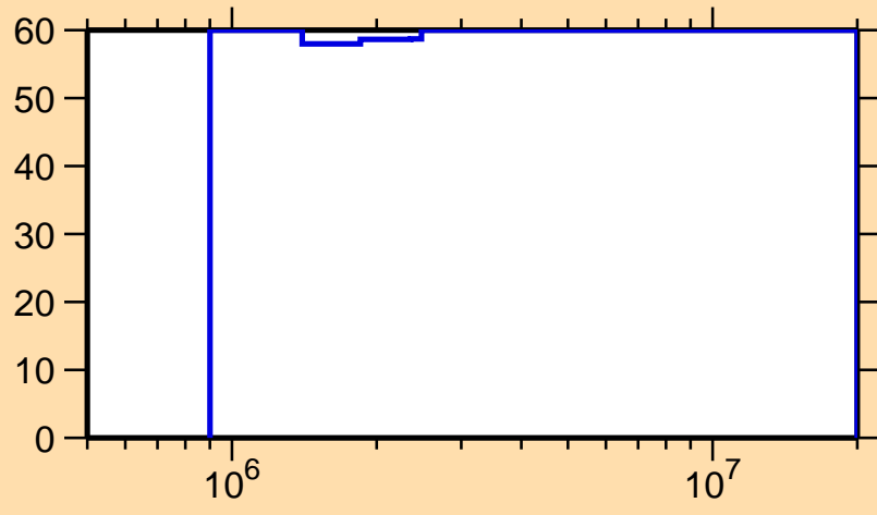
\Delta\sigma/\sigma vs. E for ^{223}\text{Ac}(n,\gamma)
