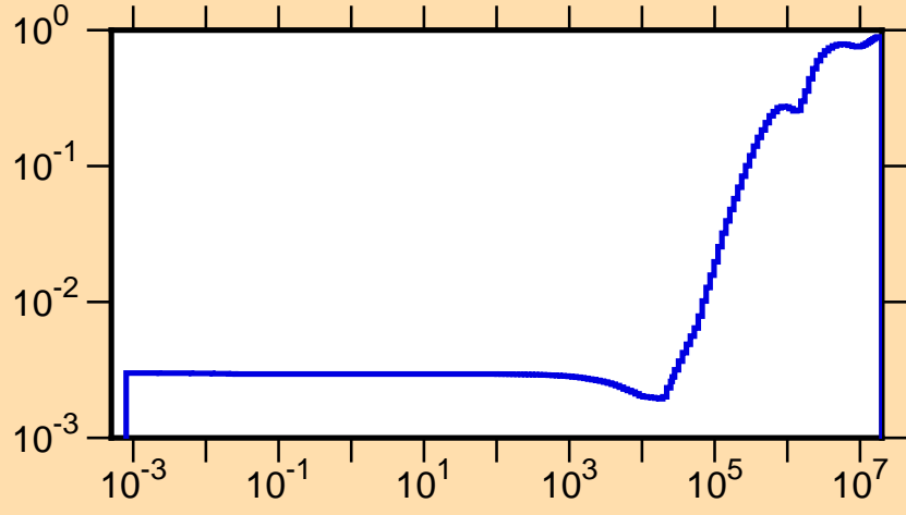
\mu vs. E for ^{224}\text{Ac}(\text{mt251})
