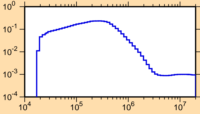
\sigma vs. E for ^{224}\text{Ac}(n,n_1)
