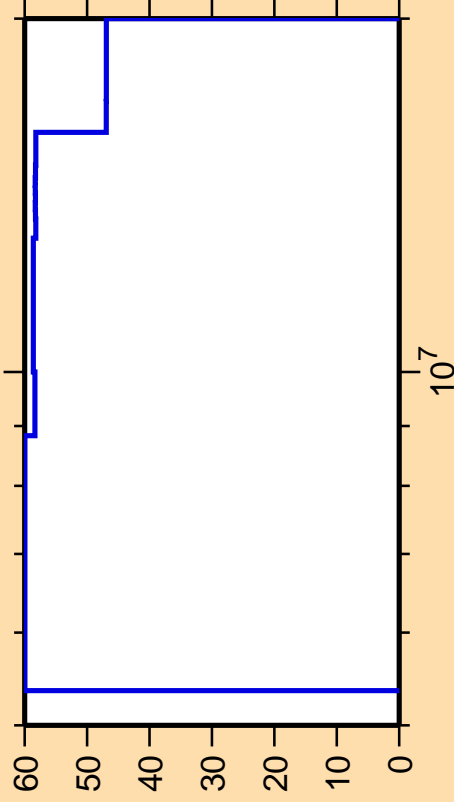
\Delta\sigma/\sigma vs. E for ^{224}\text{Ac}(n,2n)
