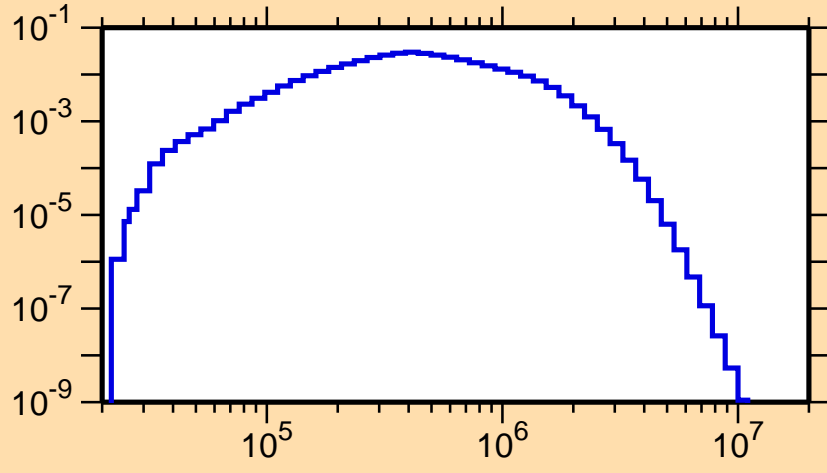
\sigma vs. E for ^{224}\text{Ac}(n,n_2)
