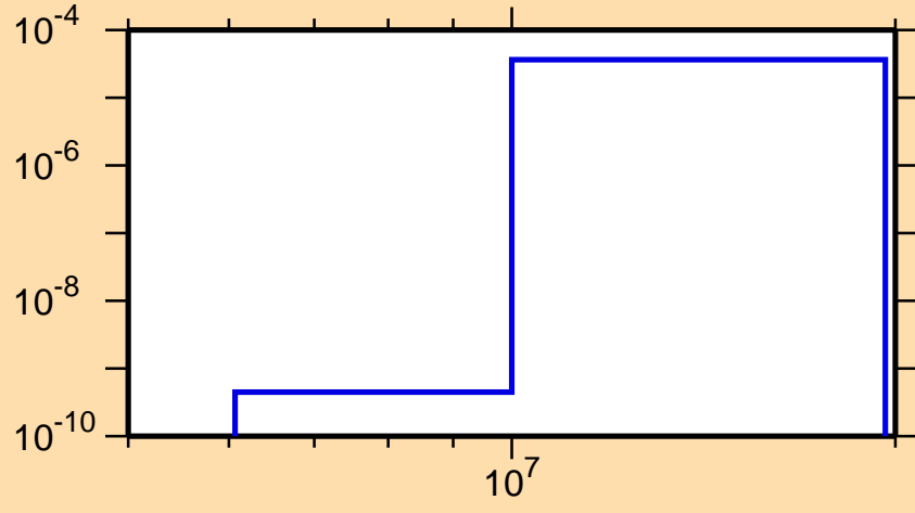
\sigma vs. E for ^{224}\text{Ac}(\text{mt117})
