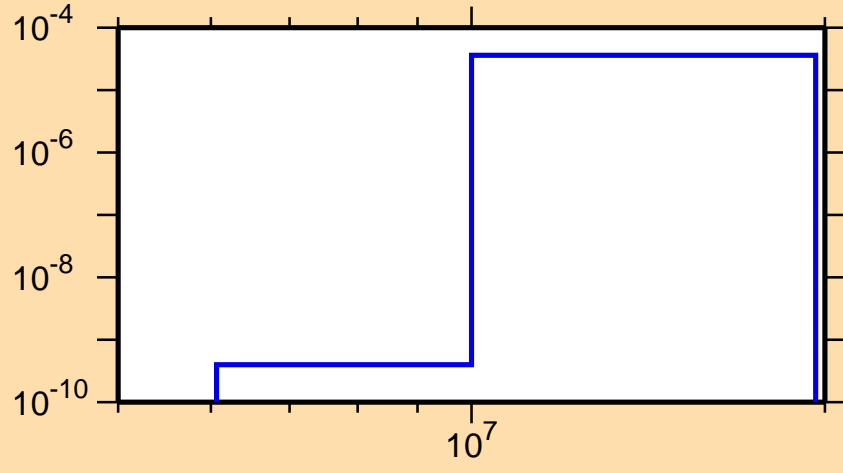
\sigma vs. E for ^{224}\text{Ac}(\text{mt } 45)
