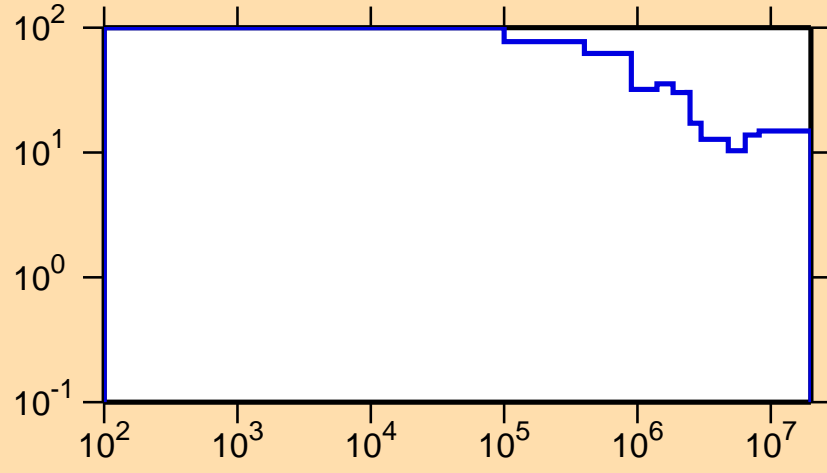
\Delta\sigma/\sigma vs. E for ^{224}\text{Ac}(n,\text{nonel.})
