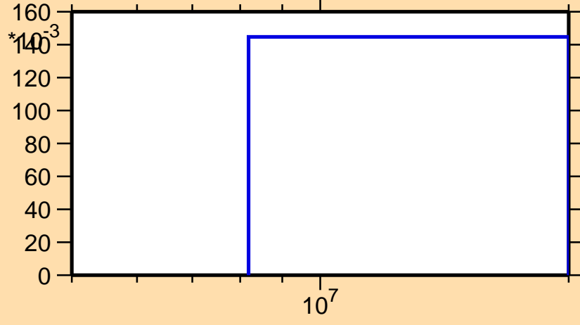
\sigma vs. E for ^{224}\text{Ac}(n,3n)
