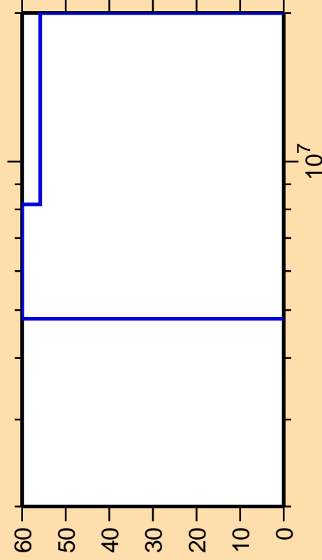
\Delta\sigma/\sigma vs. E for ^{224}\text{Ac}(n,2n)
