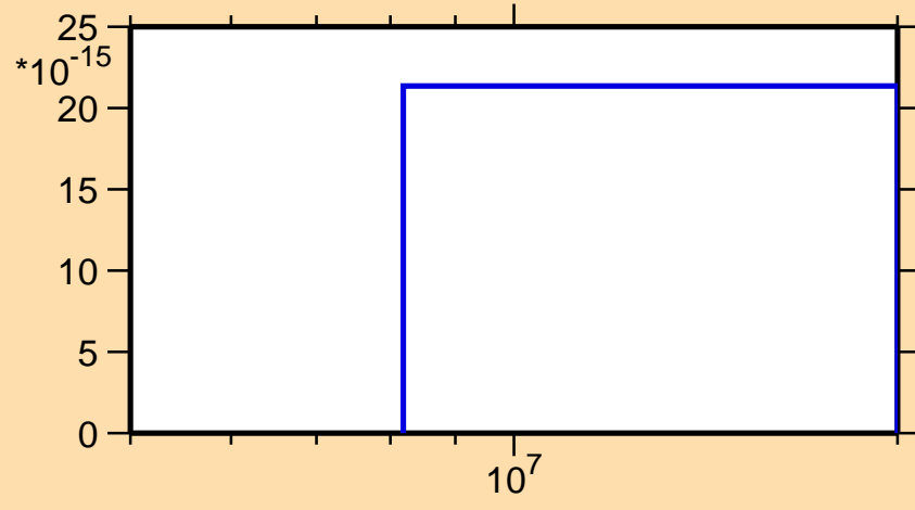
\sigma vs. E for ^{224}\text{Ac} (mt 42)
