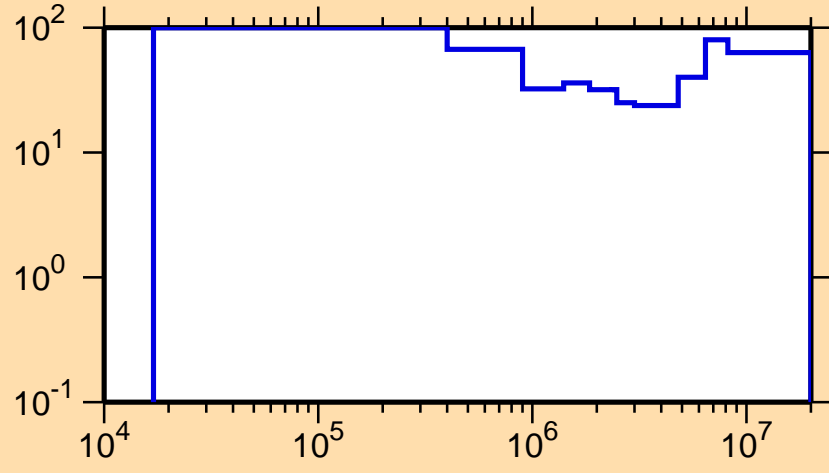
\Delta\sigma/\sigma vs. E for ^{224}\text{Ac}(n,\text{inel.})
