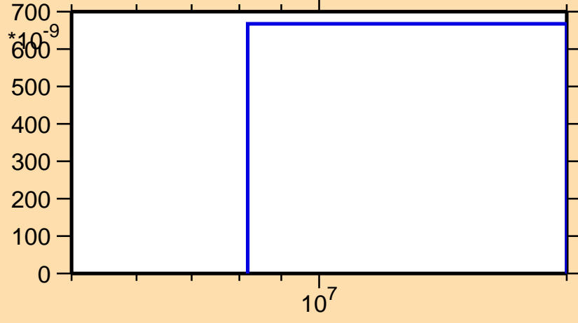
\sigma vs. E for ^{224}\text{Ac}(n,nt)
