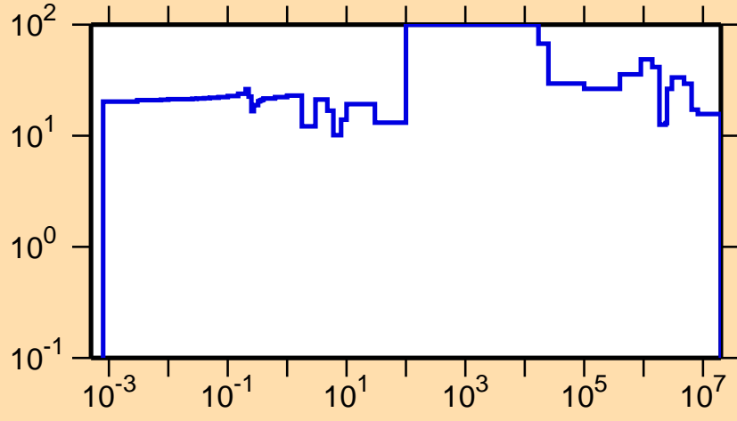
\Delta\sigma/\sigma vs. E for ^{224}\text{Ac}(n,\text{el.})
