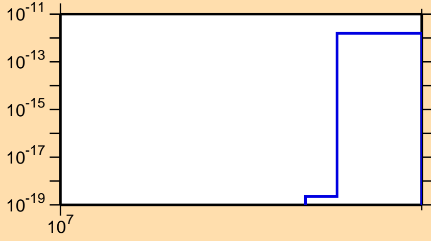
\sigma vs. E for ^{225}\text{Ac} (mt 42)
