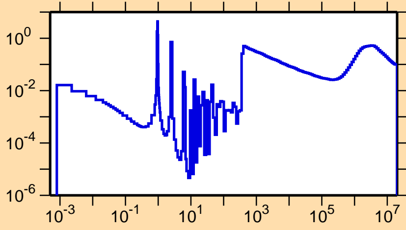
\sigma vs. E for ^{225}\text{Ac}(n,f)
