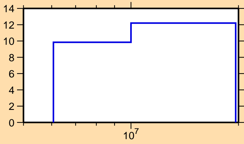
\Delta\sigma/\sigma vs. E for ^{225}\text{Ac}(n,\text{nonel.})
