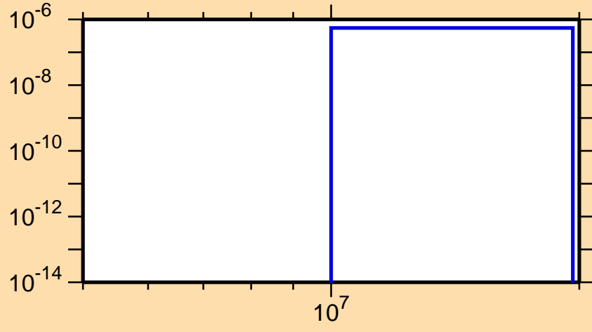
\sigma vs. E for ^{225}\text{Ac}(n,nt)
