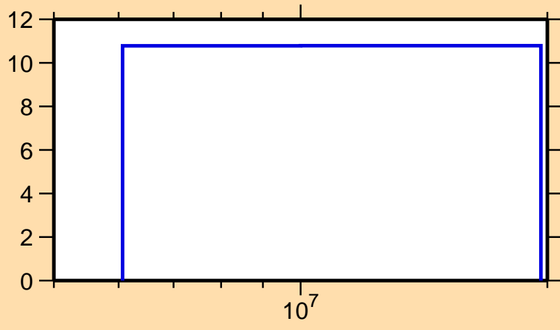
\Delta\sigma/\sigma vs. E for ^{225}\text{Ac}(n,\text{tot.})
