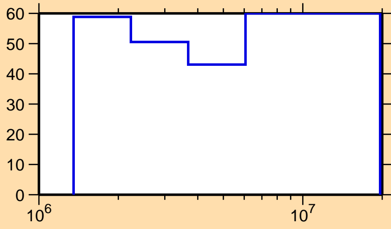
\Delta\sigma/\sigma vs. E for ^{225}\text{Ac}(n,\text{inel.})
