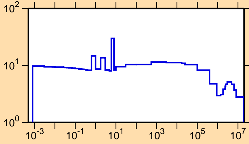
\sigma vs. E for ^{225}\text{Ac}(n,\text{el.})
