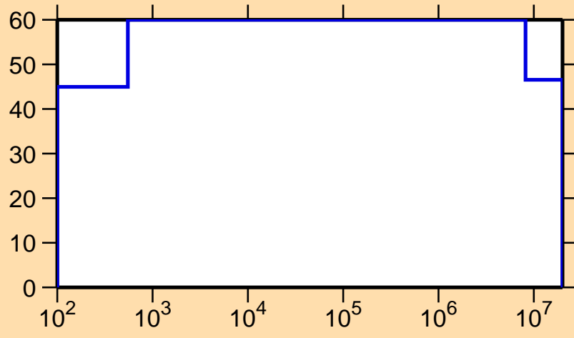
\Delta\sigma/\sigma vs. E for ^{225}\text{Ac}(n,\gamma)
