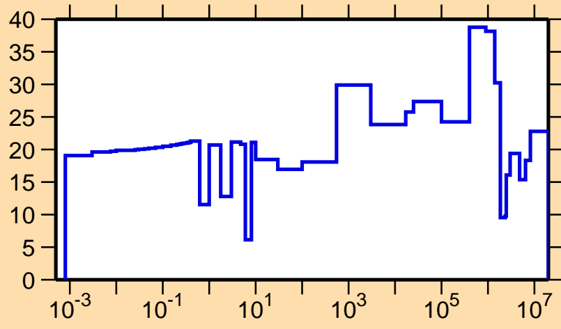
\Delta\sigma/\sigma vs. E for ^{225}\text{Ac}(n,el.)
