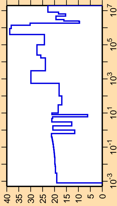
\Delta\sigma/\sigma vs. E for ^{225}\text{Ac}(n,\text{el.})
