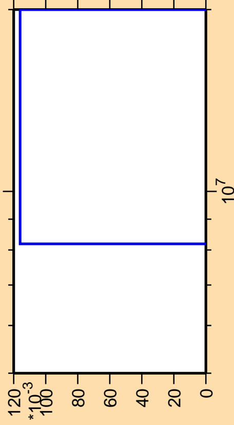
\Delta\sigma/\sigma vs. E for ^{225}\text{Ac}(\text{mt } 11)
