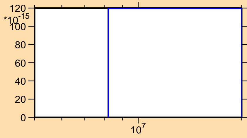
\sigma vs. E for ^{225}\text{Ac}(\text{mt } 11)
