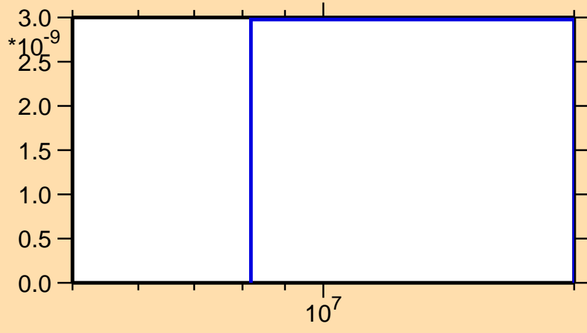
\sigma vs. E for ^{225}\text{Ac} (mt 45)
