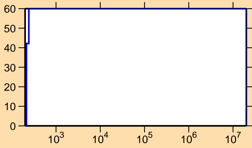
\Delta\sigma/\sigma vs. E for ^{226}\text{Ac}(n,\gamma)
