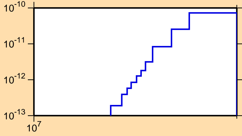
\sigma vs. E for ^{226}\text{Ac}(\text{mt117})
