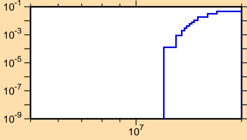
\sigma vs. E for ^{226}\text{Ac}(n,3n\alpha)
