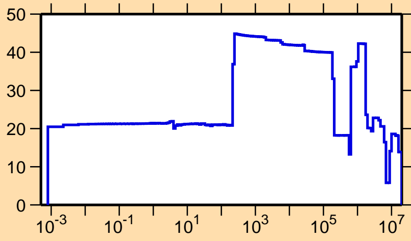
\Delta\sigma/\sigma vs. E for ^{226}\text{Ac}(n,el.)
