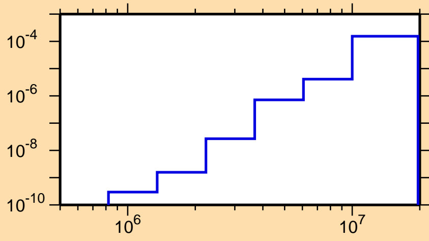
\sigma vs. E for ^{226}\text{Ac}(n,n\alpha)
