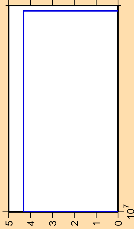
\Delta\sigma/\sigma vs. E for ^{226}\text{Ac}(\text{mt } 45)
