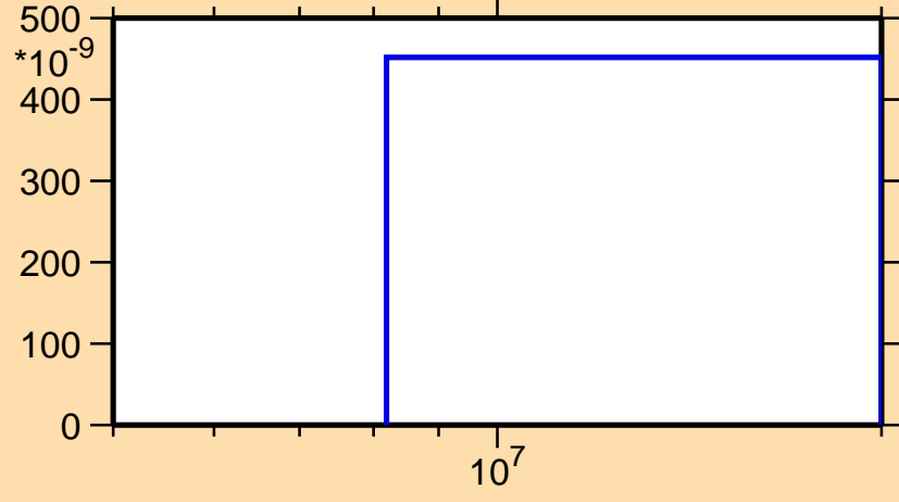
\sigma vs. E for ^{226}\text{Ac}(n,nt)
