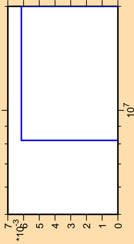
\Delta\sigma/\sigma vs. E for ^{226}\text{Ac}(\text{mt } 42)
