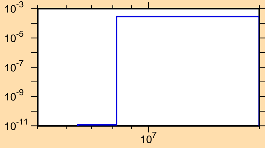
\sigma vs. E for ^{226}\text{Ac}(n,d)
