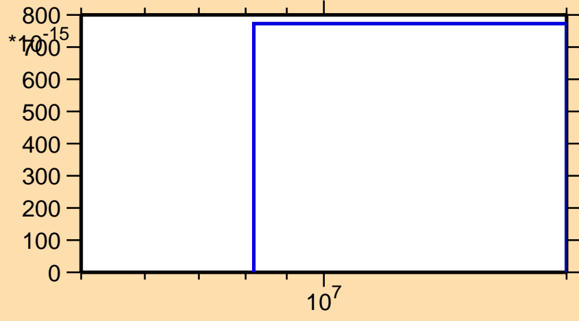
\sigma vs. E for ^{226}\text{Ac}(\text{mt } 45)
