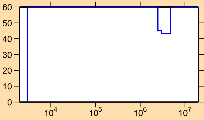
\Delta\sigma/\sigma vs. E for ^{226}\text{Ac}(n,n_1)
