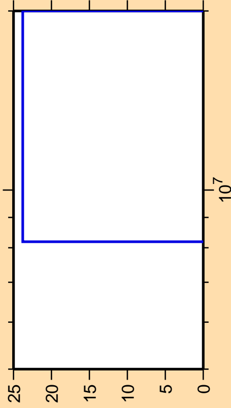
\Delta\sigma/\sigma vs. E for ^{226}\text{Ac}(\text{mt117})
