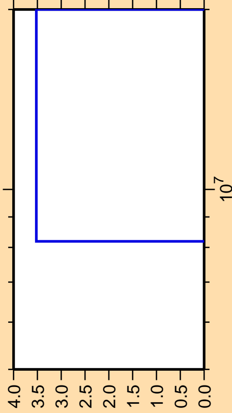
\Delta\sigma/\sigma vs. E for ^{226}\text{Ac}(\text{mt } 45)
