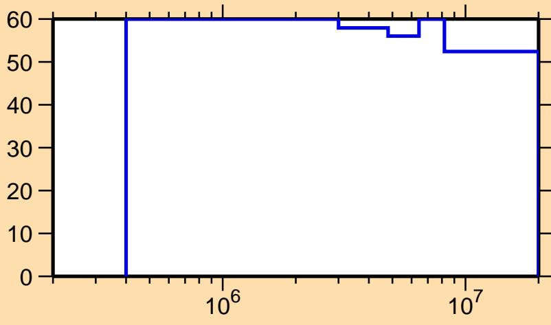
\Delta\sigma/\sigma vs. E for ^{226}\text{Ac}(n,n\text{cont.})
