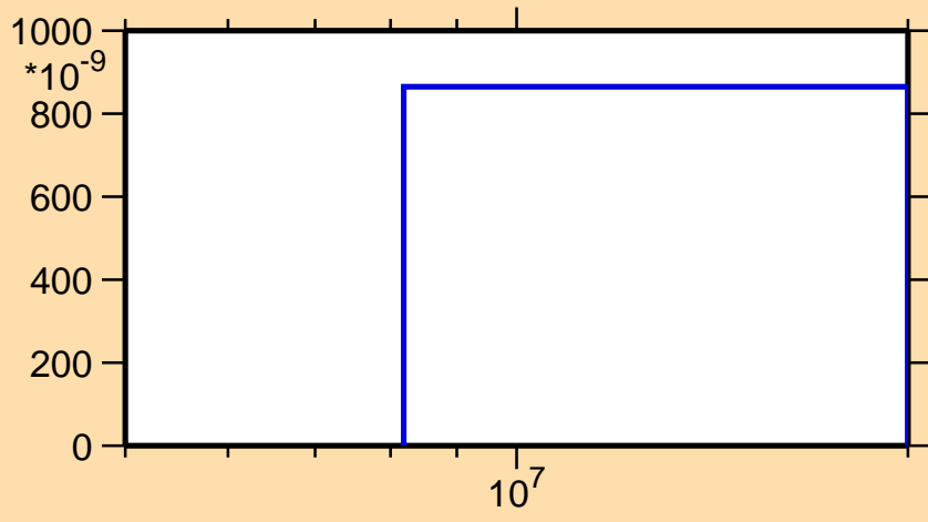
\sigma vs. E for ^{226}\text{Ac}(n,\text{nd})
