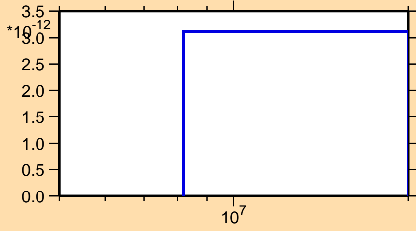
\sigma vs. E for ^{226}\text{Ac}(\text{mt117})
