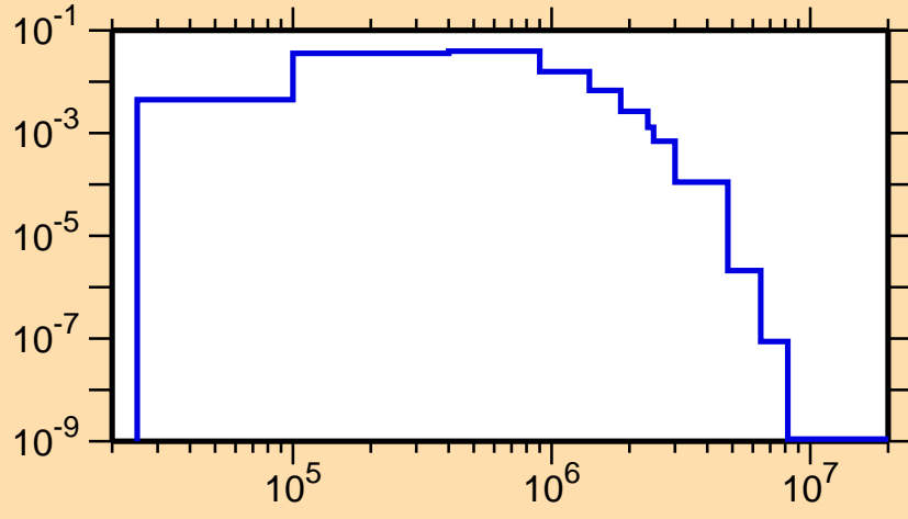
\sigma vs. E for ^{226}\text{Ac}(n,n_3)
