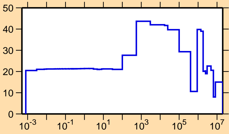
\Delta\sigma/\sigma vs. E for ^{226}\text{Ac}(n,\text{el.})
