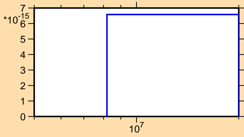
\sigma vs. E for ^{226}\text{Ac}(\text{mt } 42)
