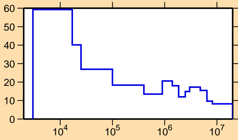
\Delta\sigma/\sigma vs. E for ^{226}\text{Ac}(n,\text{tot.})
