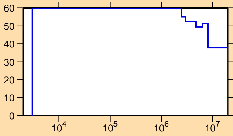
\Delta\sigma/\sigma vs. E for ^{226}\text{Ac}(n,\text{inel.})
