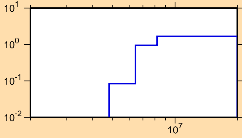
\sigma vs. E for ^{226}\text{Ac}(n,2n)
