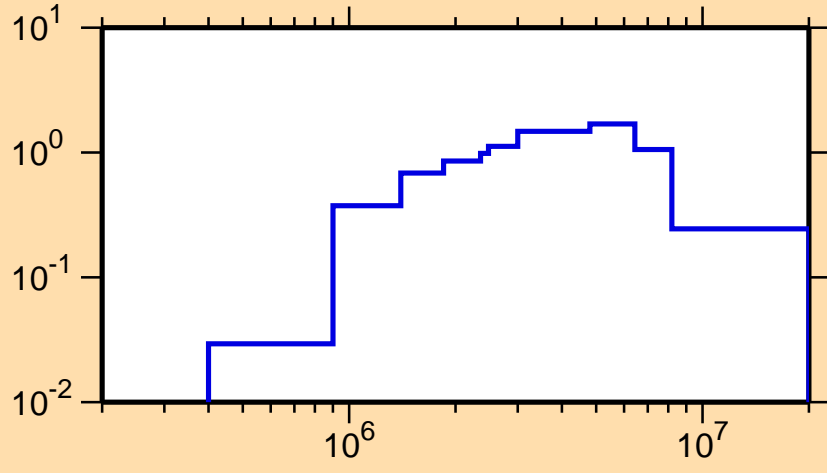
\sigma vs. E for ^{226}\text{Ac}(n,n\text{cont.})
