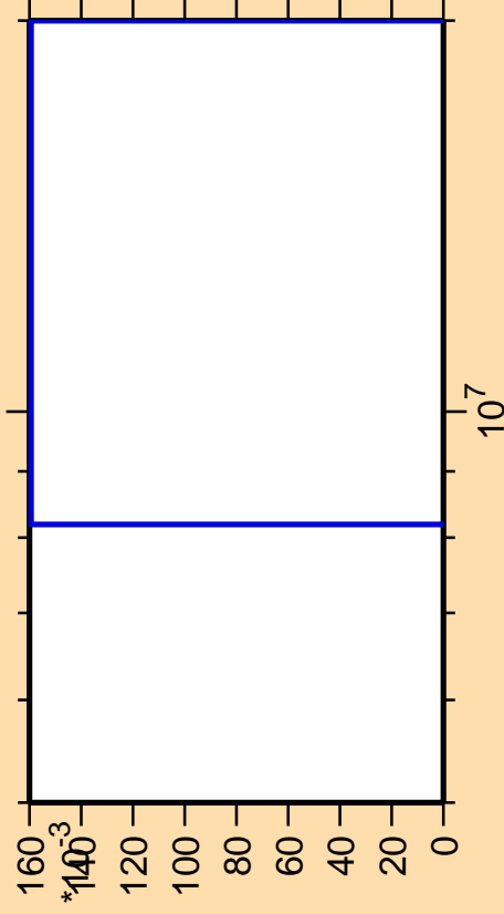
\Delta\sigma/\sigma vs. E for ^{226}\text{Ac}(\text{mt } 11)
