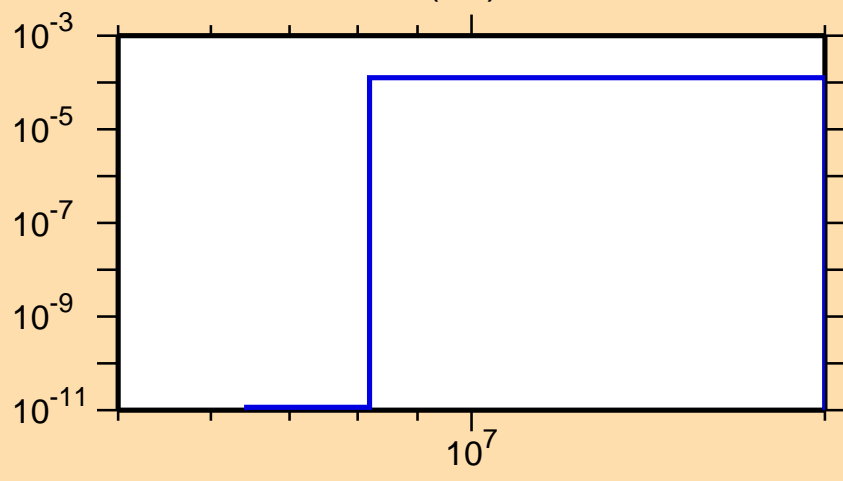
\sigma vs. E for ^{226}\text{Ac}(n,t)
