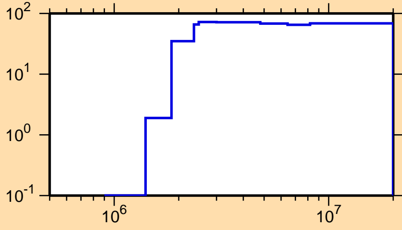
\Delta\sigma/\sigma vs. E for ^{226}\text{Ac}(n,p)
