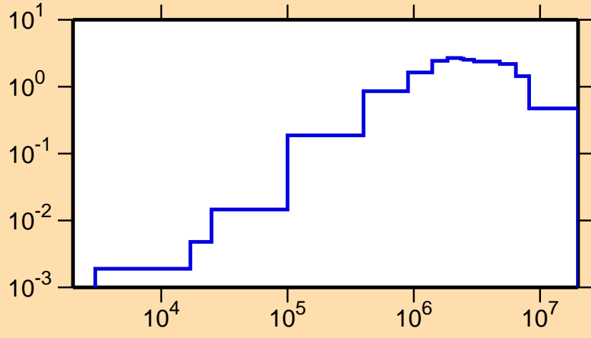
\sigma vs. E for ^{226}\text{Ac}(n,\text{inel.})
