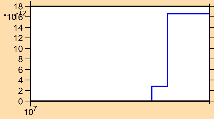
\sigma vs. E for ^{227}\text{Ac} (mt 45)
