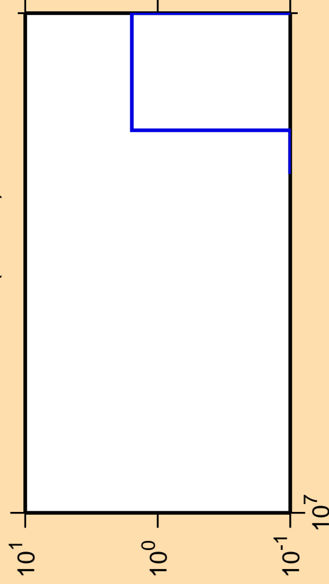
\Delta\sigma/\sigma vs. E for ^{227}\text{Ac} (mt 42)
