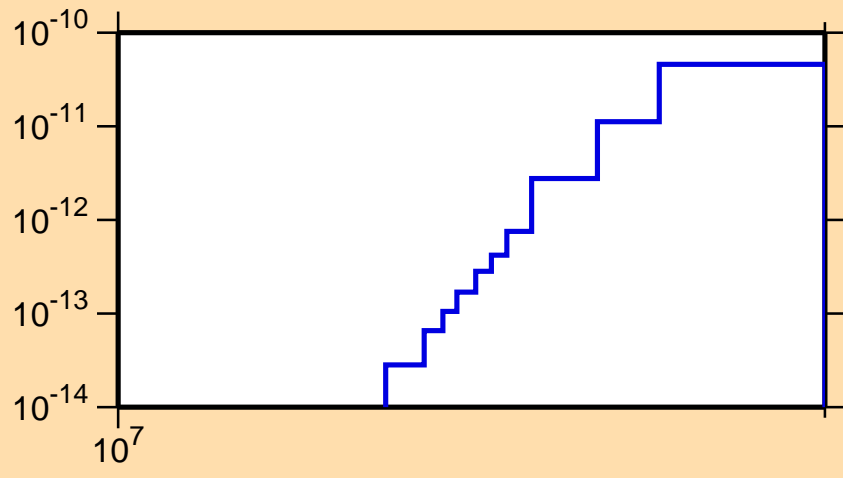
\sigma vs. E for ^{227}\text{Ac}(\text{mt117})
