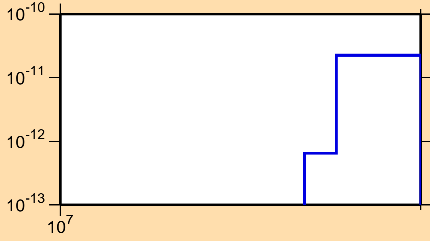
\sigma vs. E for ^{227}\text{Ac}(n,\text{He3})
