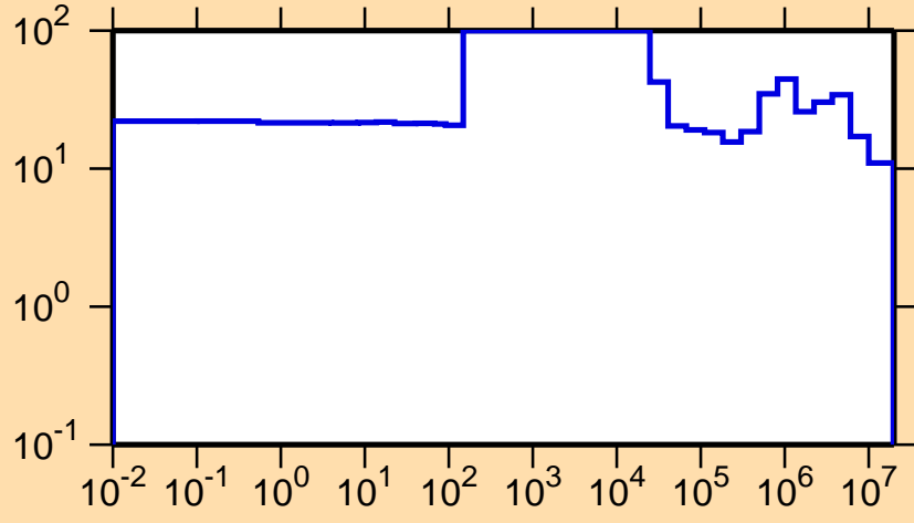
\Delta\sigma/\sigma vs. E for ^{227}\text{Ac}(n,el.)
