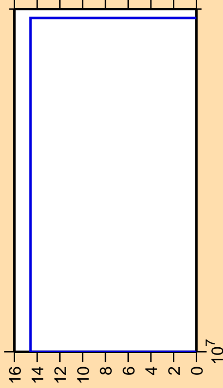
\Delta\sigma/\sigma vs. E for ^{227}\text{Ac}(n,p\alpha)
