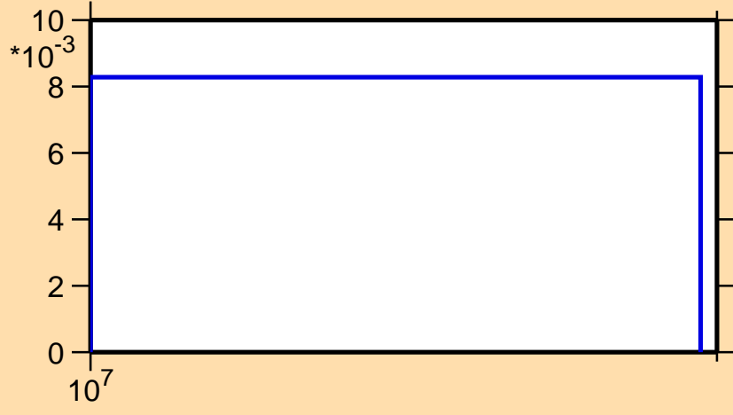
\sigma vs. E for ^{227}\text{Ac}(n,3n\alpha)
