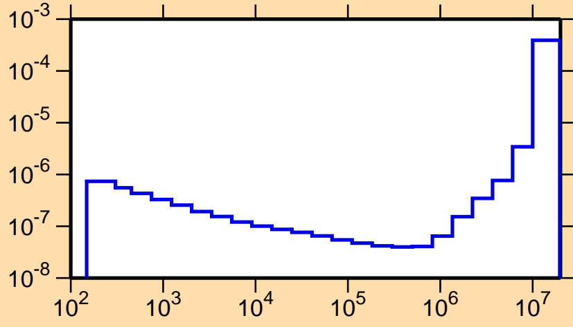
\sigma vs. E for ^{227}\text{Ac}(n,\alpha)
