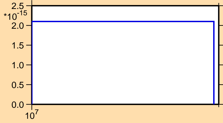
\sigma vs. E for ^{227}\text{Ac} (mt 42)
