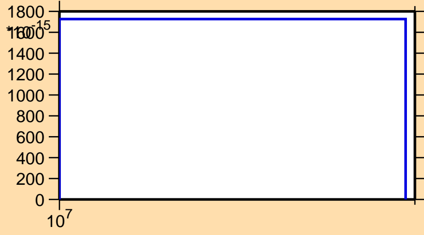
\sigma vs. E for ^{227}\text{Ac}(n,p\alpha)
