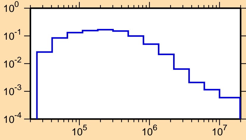
\sigma vs. E for ^{227}\text{Ac}(n,n_1)
