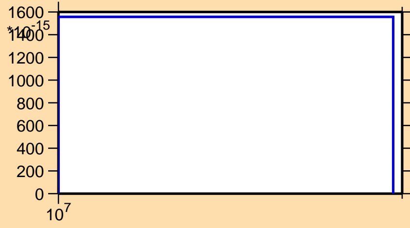
\sigma vs. E for ^{227}\text{Ac}(\text{mt117})
