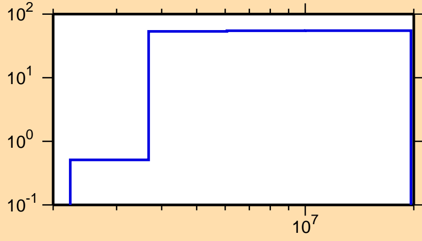
\Delta\sigma/\sigma vs. E for ^{227}\text{Ac}(n,p)
