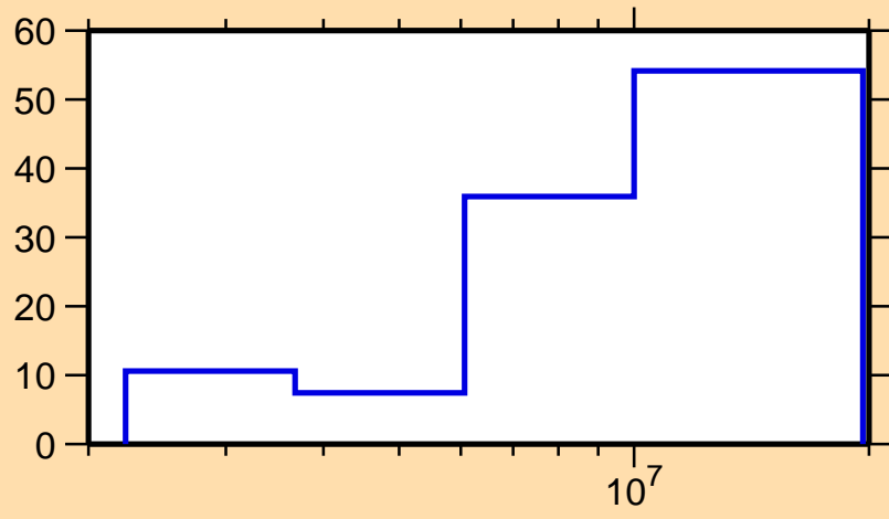
\Delta\sigma/\sigma vs. E for ^{227}\text{Ac}(n,n\text{cont.})
