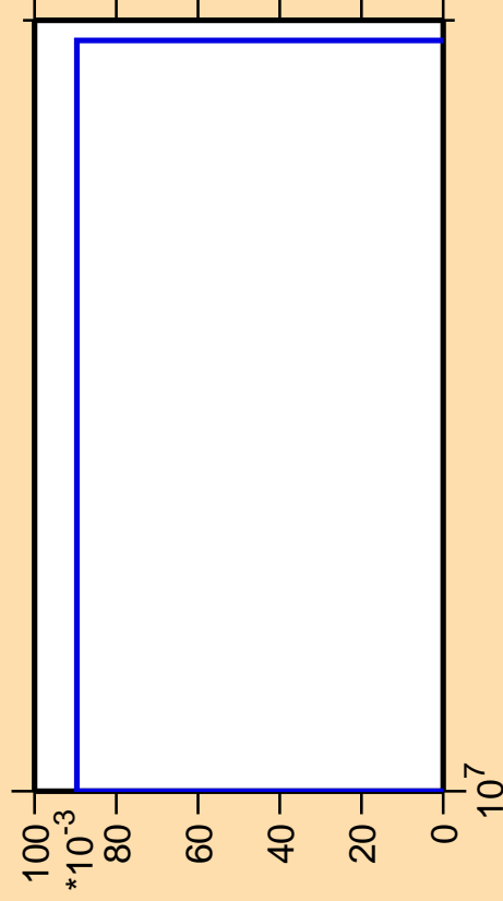
\Delta\sigma/\sigma vs. E for ^{227}\text{Ac} (mt 11)
