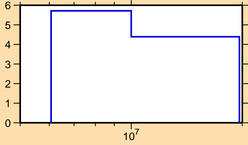
\Delta\sigma/\sigma vs. E for ^{227}\text{Ac}(n,\text{nonel.})
