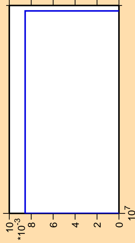
\Delta\sigma/\sigma vs. E for ^{227}\text{Ac} (mt 42)
