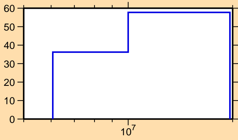
\Delta\sigma/\sigma vs. E for ^{227}\text{Ac}(n,2n)
