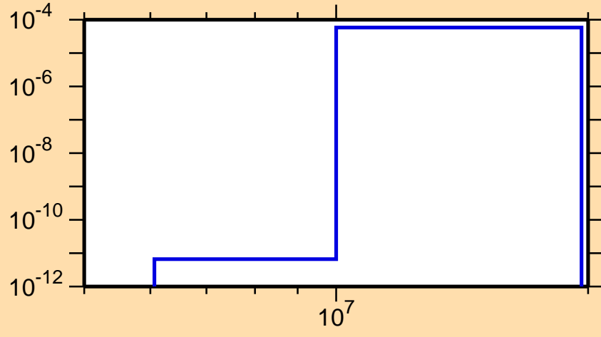
\sigma vs. E for ^{227}\text{Ac}(n,t)
