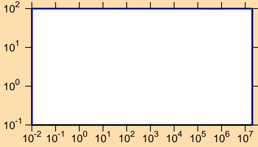
\Delta\sigma/\sigma vs. E for ^{227}\text{Ac}(n,f)
