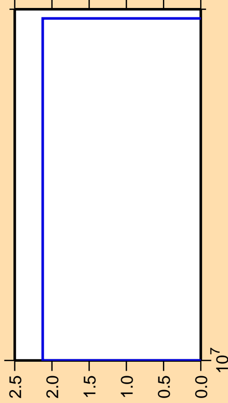
\Delta\sigma/\sigma vs. E for ^{227}\text{Ac} (mt 45)
