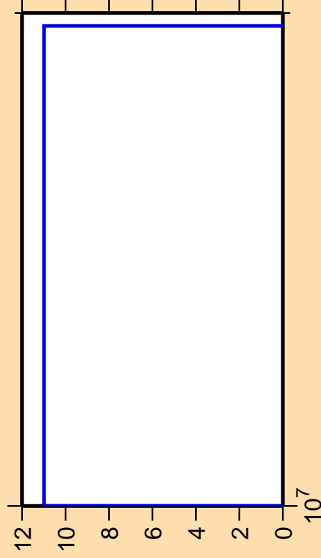
\Delta\sigma/\sigma vs. E for ^{227}\text{Ac}(\text{mt117})
