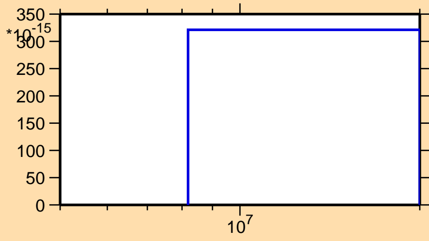
\sigma vs. E for ^{227}\text{Ac}(\text{mt } 45)
