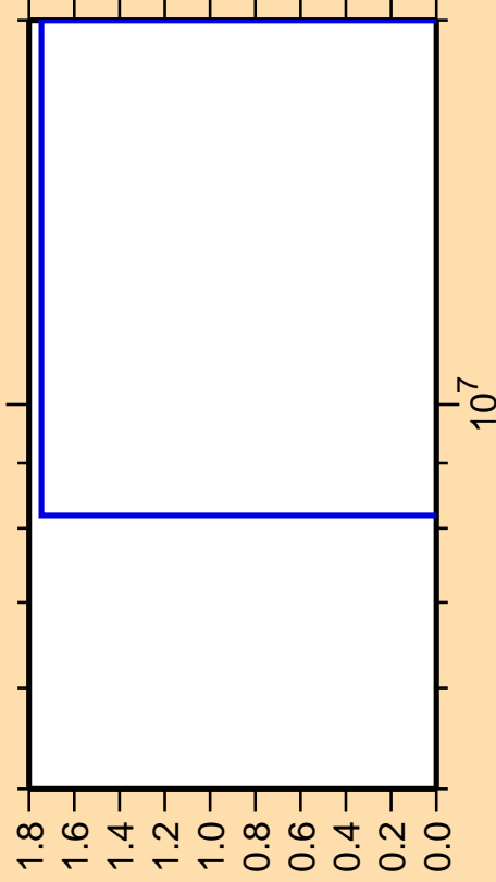
\Delta\sigma/\sigma vs. E for ^{227}\text{Ac}(\text{mt } 45)
