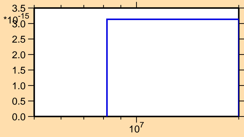
\sigma vs. E for ^{227}\text{Ac} (mt 42)
