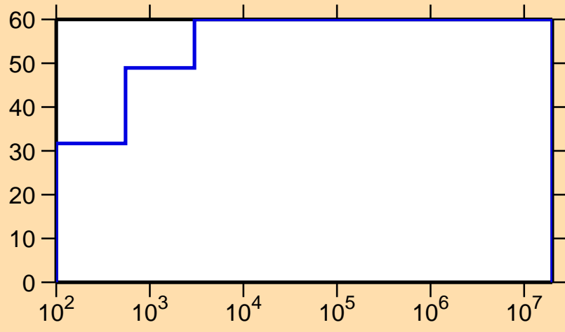
\Delta\sigma/\sigma vs. E for ^{227}\text{Ac}(n,\gamma)
