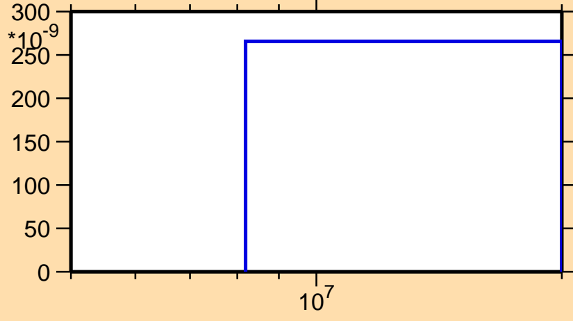
\sigma vs. E for ^{227}\text{Ac}(n,nt)
