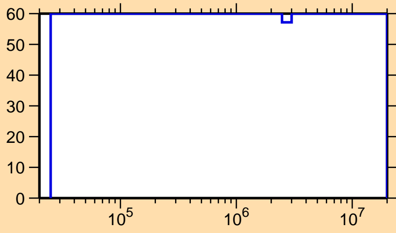
\Delta\sigma/\sigma vs. E for ^{227}\text{Ac}(n,n_1)
