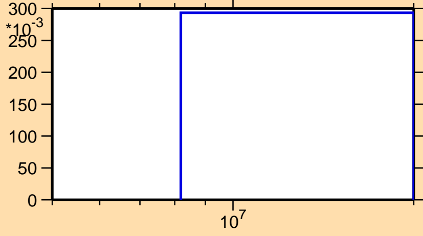
\sigma vs. E for ^{227}\text{Ac}(n,3n)
