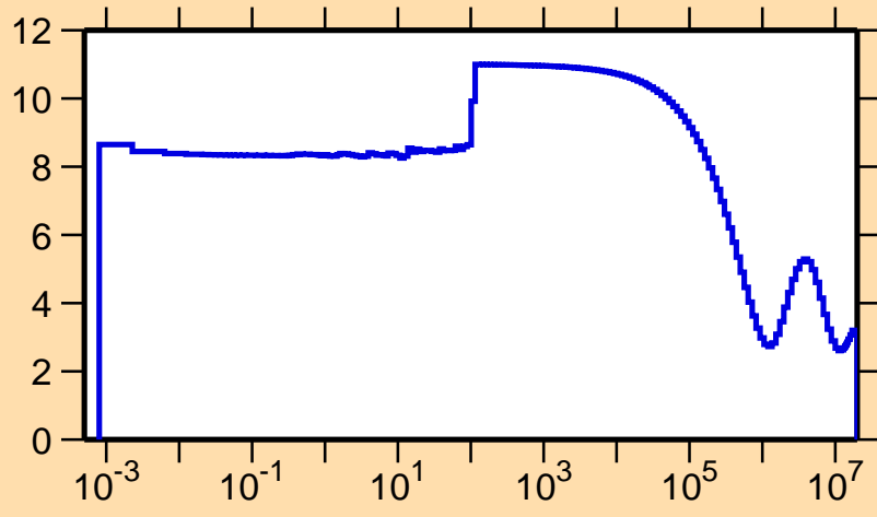
\sigma vs. E for ^{228}\text{Ac}(n,\text{el.})
