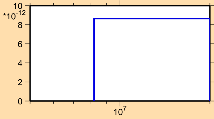
\sigma vs. E for ^{228}\text{Ac}(n,p\alpha)
