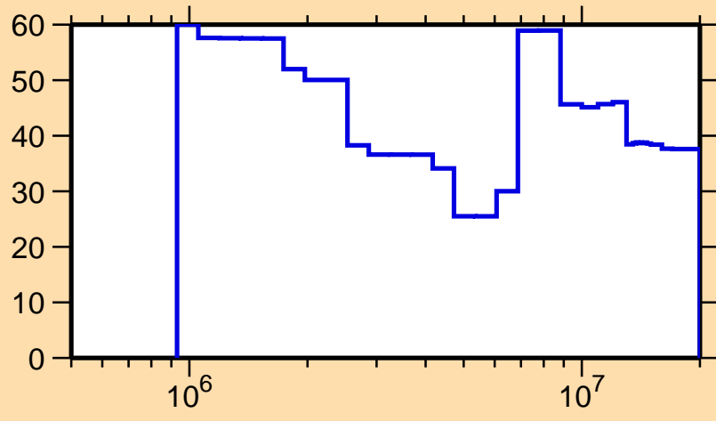
\Delta\sigma/\sigma vs. E for ^{229}\text{Ac}(n,\text{inel.})
