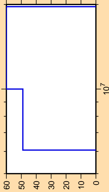
\Delta\sigma/\sigma vs. E for ^{229}\text{Ac}(n,2n)
