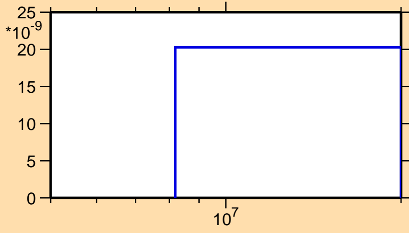
\sigma vs. E for ^{229}\text{Ac}(n,\text{nd})
