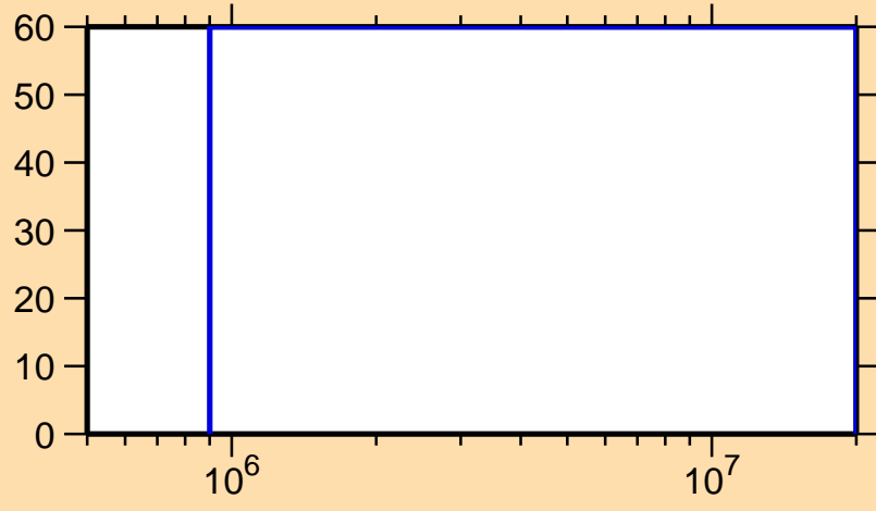
\Delta\sigma/\sigma vs. E for ^{229}\text{Ac}(n,n_1)
