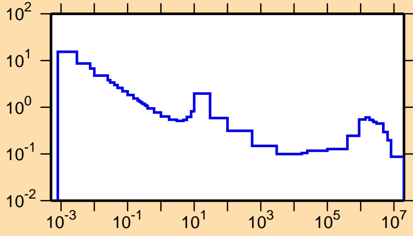
\sigma vs. E for ^{229}\text{Ac}(n,f)
