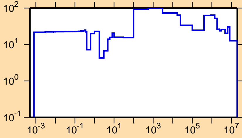
\Delta\sigma/\sigma vs. E for ^{229}\text{Ac}(n,\text{el.})
