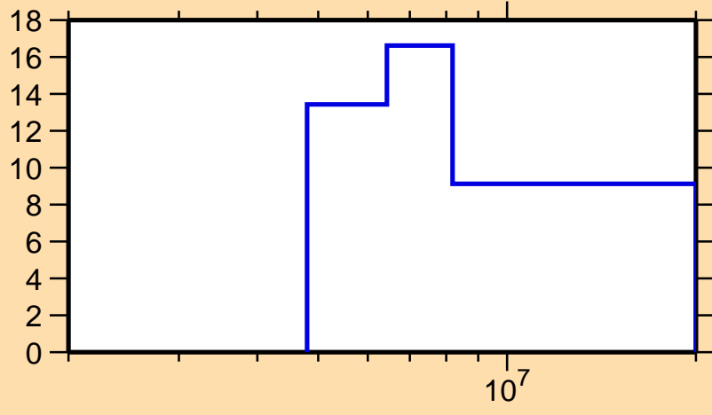
\Delta\sigma/\sigma vs. E for ^{229}\text{Ac}(n,\text{tot.})
