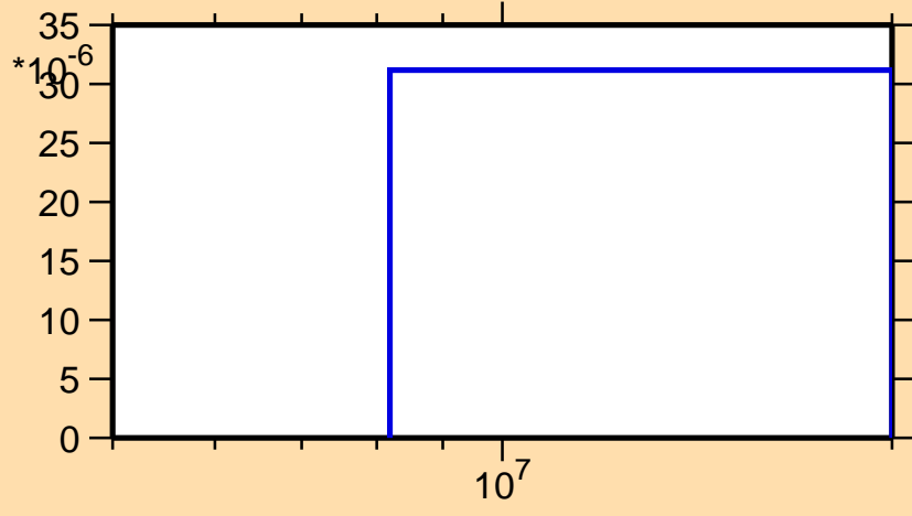
\sigma vs. E for ^{229}\text{Ac}(n,t)
