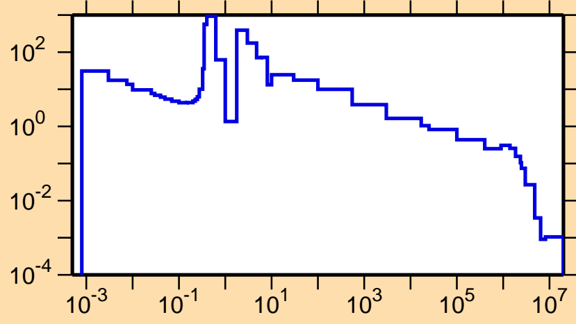
\sigma vs. E for ^{229}\text{Ac}(n,\gamma)
