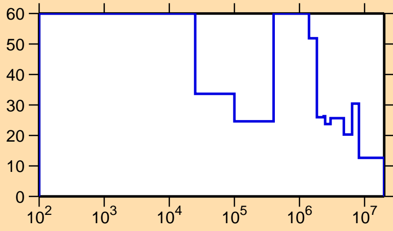
\Delta\sigma/\sigma vs. E for ^{229}\text{Ac}(n,\text{el.})
