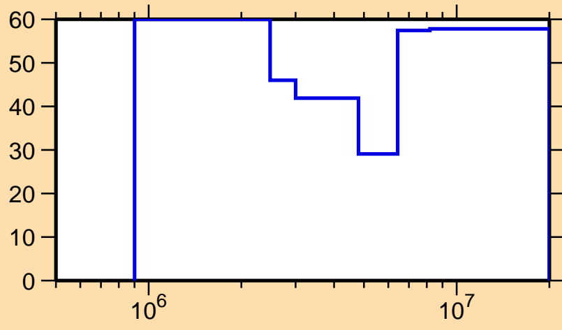
\Delta\sigma/\sigma vs. E for ^{229}\text{Ac}(n,n\text{cont.})
