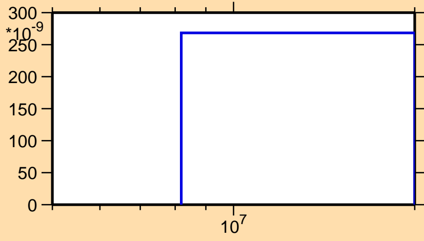
\sigma vs. E for ^{229}\text{Ac}(n,nt)
