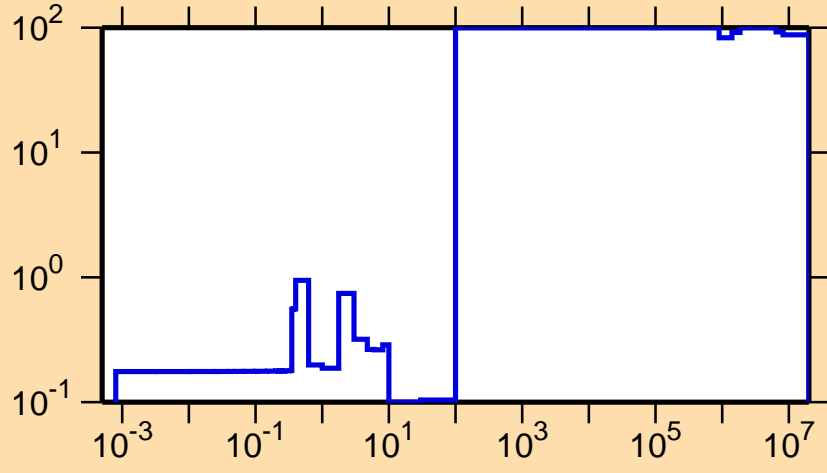
\Delta\sigma/\sigma vs. E for ^{229}\text{Ac}(n,f)
