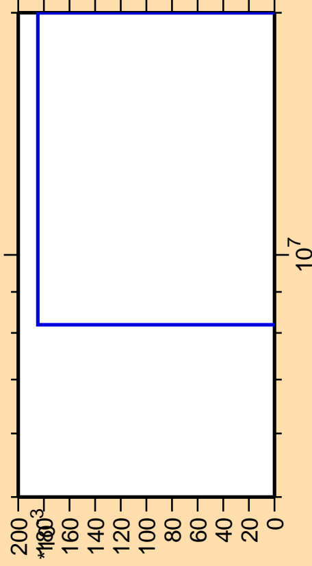
\Delta\sigma/\sigma vs. E for ^{229}\text{Ac}(\text{mt } 11)
