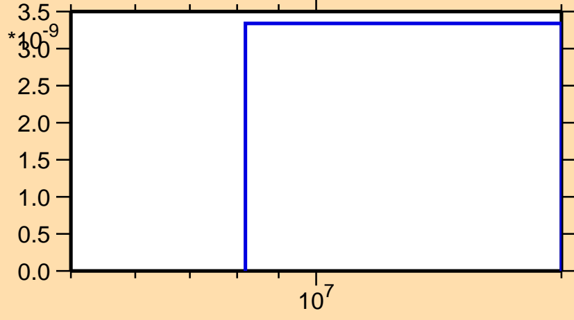
\sigma vs. E for ^{229}\text{Ac}(n,2np)
