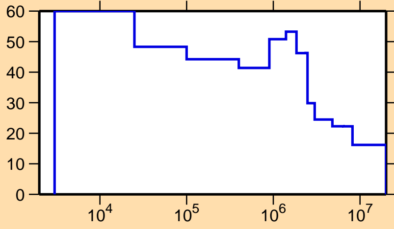
\Delta\sigma/\sigma vs. E for ^{229}\text{Ac}(n,\text{nonel.})
