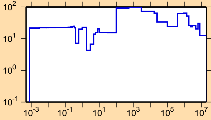
\Delta\sigma/\sigma vs. E for ^{229}\text{Ac}(n,el.)
