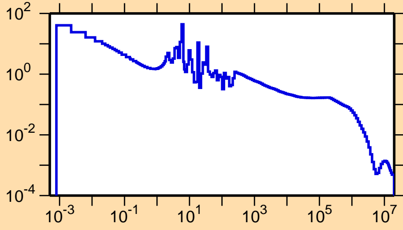
\sigma vs. E for ^{230}\text{Ac}(n,\gamma)
