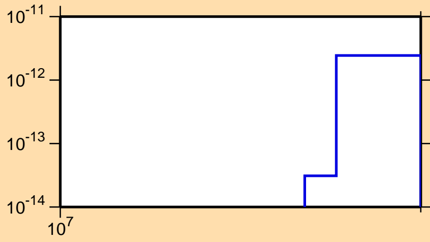
\sigma vs. E for ^{230}\text{Ac}(n,\text{He3})
