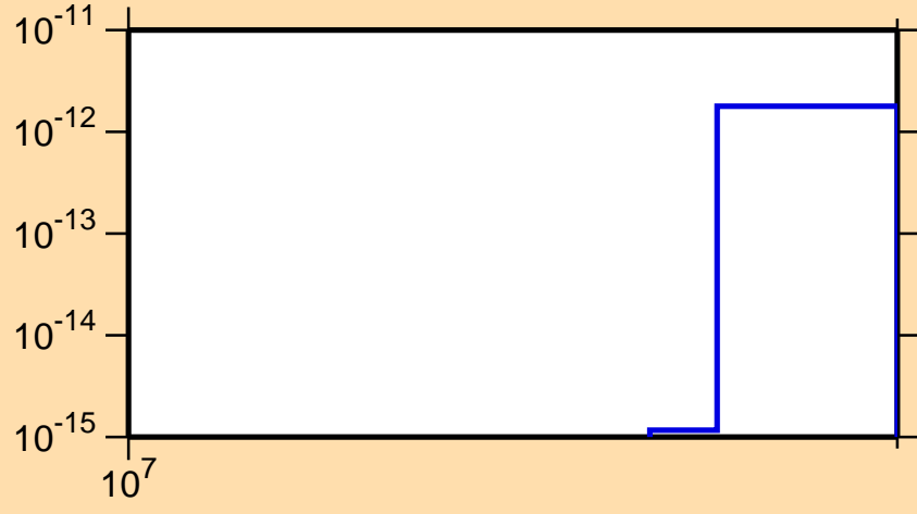
\sigma vs. E for ^{230}\text{Ac} (mt 11)
