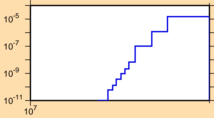
\sigma vs. E for ^{230}\text{Ac}(n,nt)
