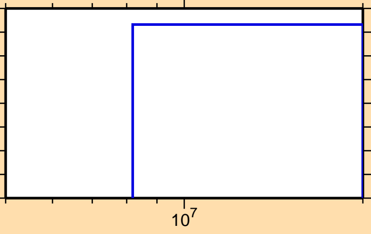
\sigma vs. E for ^{230}\text{Ac} (mt 11)
