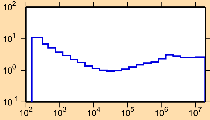
\sigma vs. E for ^{231}\text{Ac}(n,\text{nonel.})
