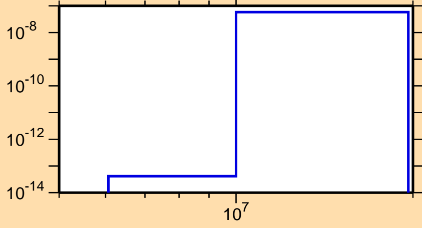
\sigma vs. E for ^{231}\text{Ac}(n,2n\alpha)
