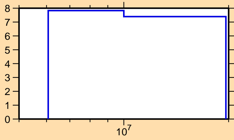
\Delta\sigma/\sigma vs. E for ^{231}\text{Ac}(n,\text{nonel.})
