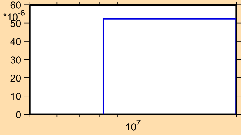
\sigma vs. E for ^{231}\text{Ac}(n,d)
