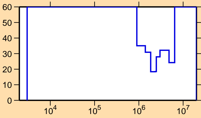
\Delta\sigma/\sigma vs. E for ^{231}\text{Ac}(n,\text{inel.})
