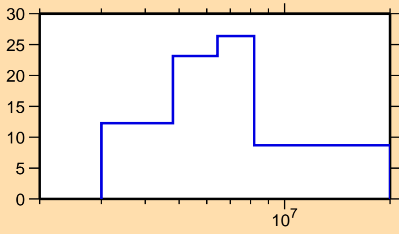
\Delta\sigma/\sigma vs. E for ^{231}\text{Ac}(n,\text{tot.})
