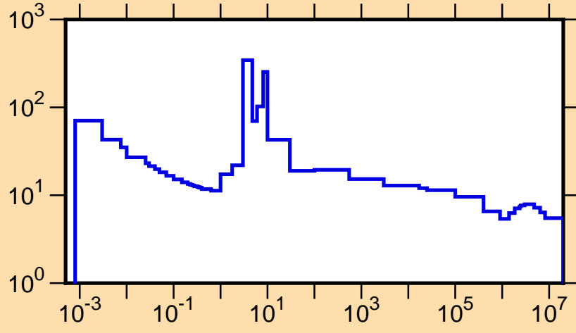
\sigma vs. E for ^{231}\text{Ac}(n,\text{tot.})
