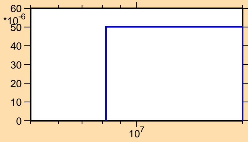
\sigma vs. E for ^{231}\text{Ac}(n,np)
