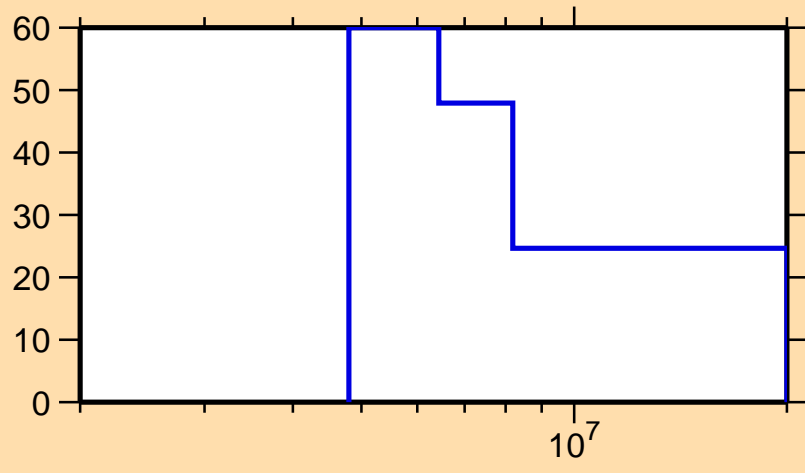
\Delta\sigma/\sigma vs. E for ^{231}\text{Ac}(n,2n)
