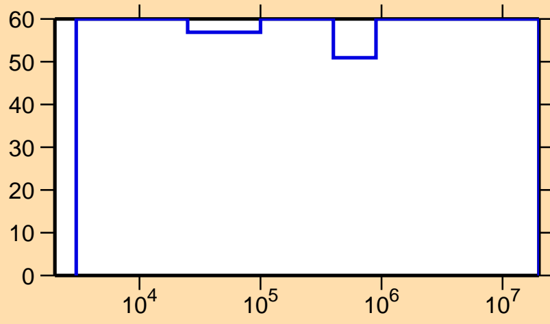
\Delta\sigma/\sigma vs. E for ^{231}\text{Ac}(n,n_1)
