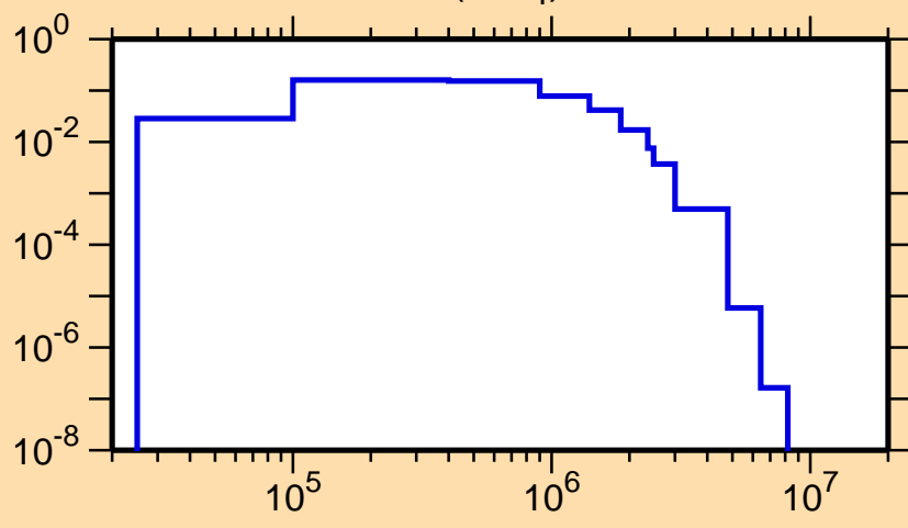
\sigma vs. E for ^{231}\text{Ac}(n,n_4)
