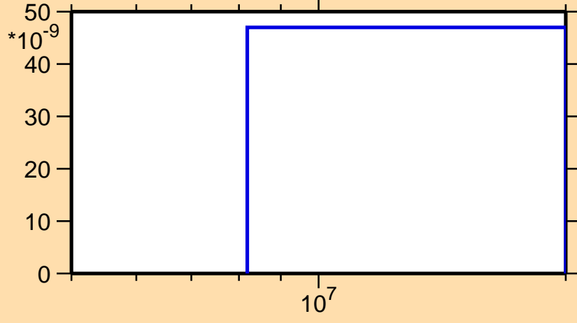
\sigma vs. E for ^{231}\text{Ac}(n,2n\alpha)
