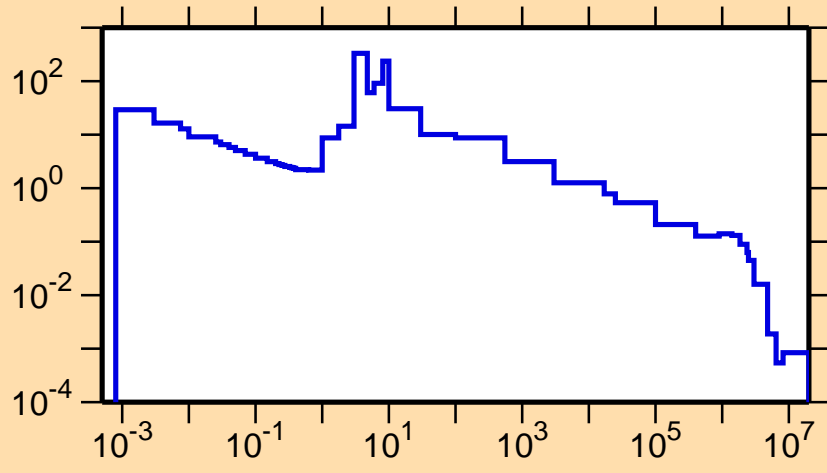
\sigma vs. E for ^{231}\text{Ac}(n,\gamma)
