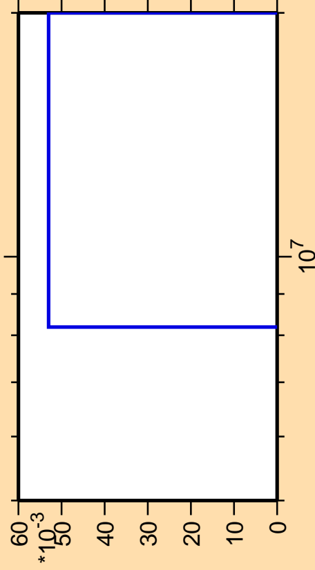
\Delta\sigma/\sigma vs. E for ^{231}\text{Ac}(\text{mt } 11)
