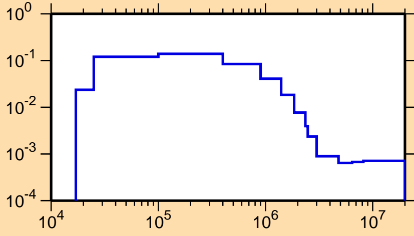
\sigma vs. E for ^{231}\text{Ac}(n,n_2)
