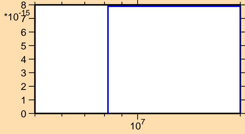
\sigma vs. E for ^{231}\text{Ac}(\text{mt } 11)
