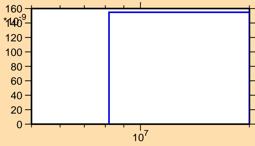
\sigma vs. E for ^{231}\text{Ac}(n,nt)
