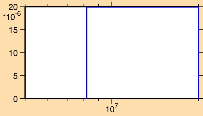
\sigma vs. E for ^{231}\text{Ac}(n,t)
