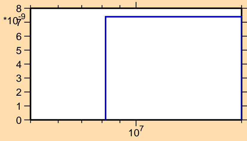
\sigma vs. E for ^{231}\text{Ac}(n,\text{nd})
