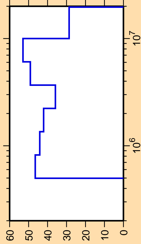
\Delta\sigma/\sigma vs. E for ^{232}\text{Ac}(n,n\text{cont.})
