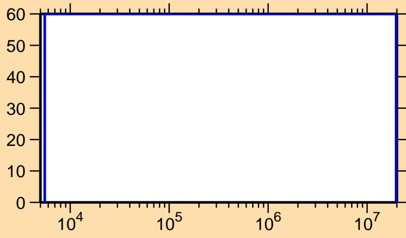
\Delta\sigma/\sigma vs. E for ^{232}\text{Ac}(n,f)
