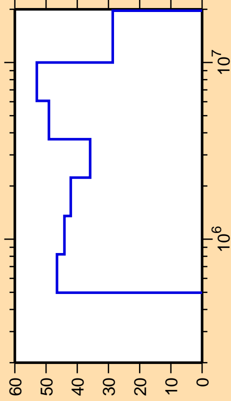
\Delta\sigma/\sigma vs. E for ^{232}\text{Ac}(n,\text{ncont.})
