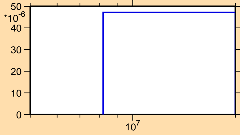
\sigma vs. E for ^{232}\text{Ac}(n,t)
