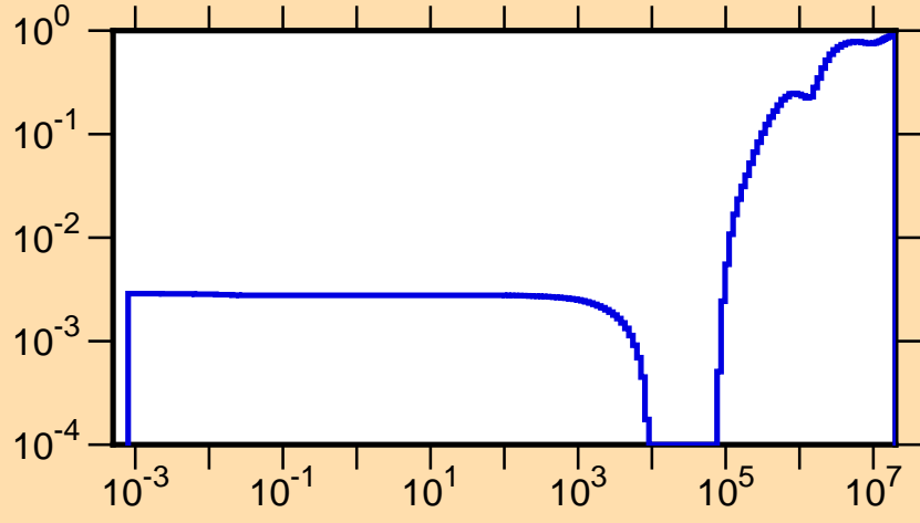
\mu vs. E for ^{233}\text{Ac}(\text{mt251})
