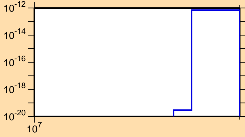
\sigma vs. E for ^{233}\text{Ac}(\text{mt } 11)
