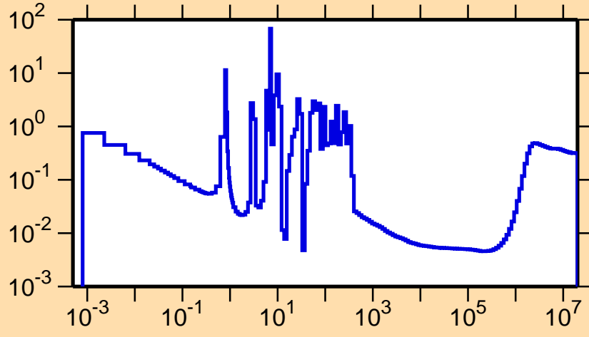
\sigma vs. E for ^{233}\text{Ac}(n,f)
