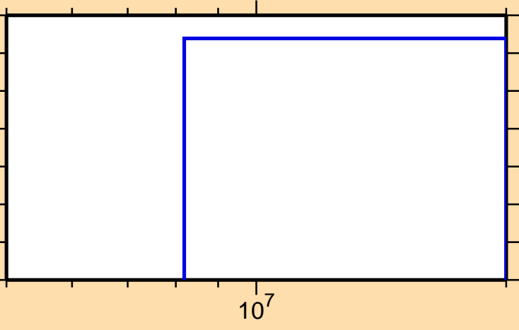
\sigma vs. E for ^{233}\text{Ac}(n,d)
