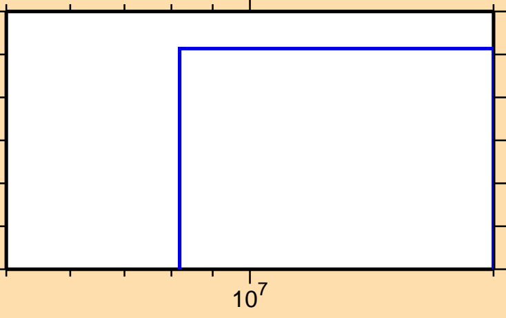
\sigma vs. E for ^{233}\text{Ac}(n,\text{nd})
