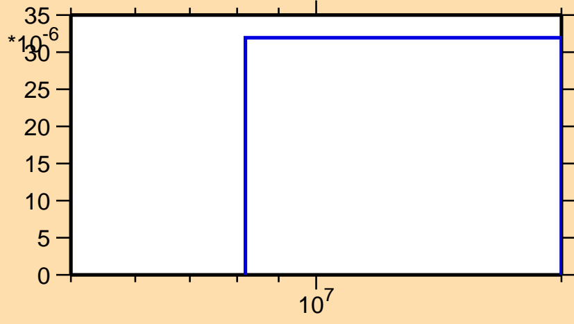
\sigma vs. E for ^{233}\text{Ac}(n,d)
