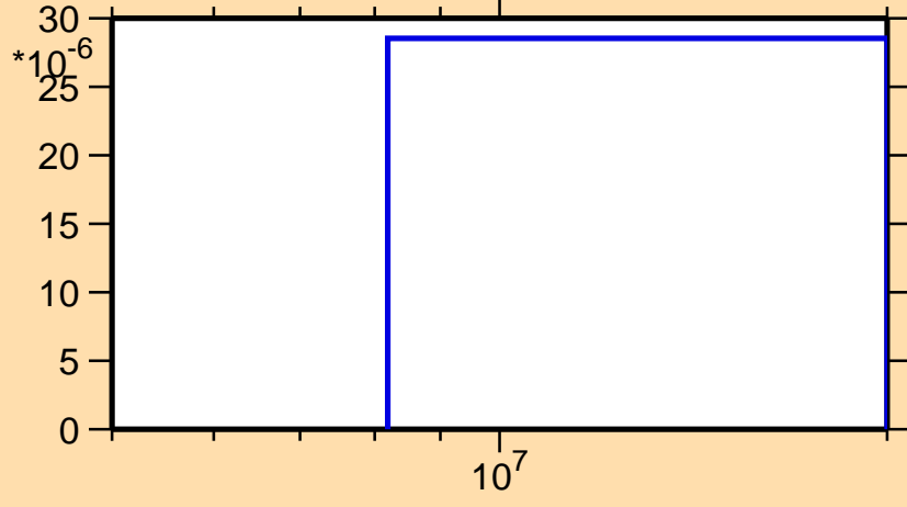
\sigma vs. E for ^{233}\text{Ac}(n,np)
