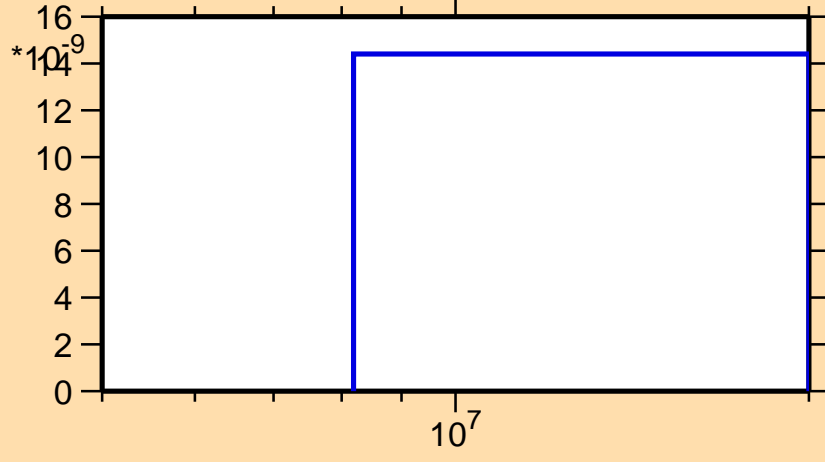
\sigma vs. E for ^{233}\text{Ac}(n,2n\alpha)
