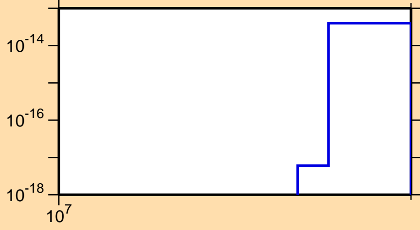
\sigma vs. E for ^{234}\text{Ac}(n,\text{He3})
