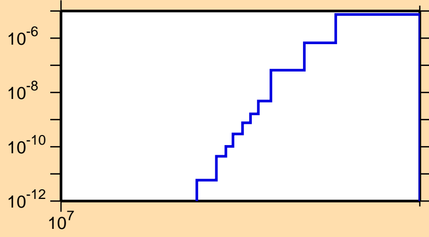
\sigma vs. E for ^{234}\text{Ac}(n,\text{nd})
