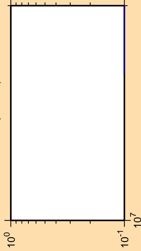
\Delta\sigma/\sigma vs. E for ^{234}\text{Ac}(n,\text{He3})
