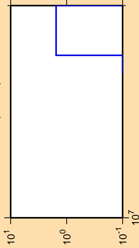
\Delta\sigma/\sigma vs. E for ^{234}\text{Ac}(\text{mt } 11)
