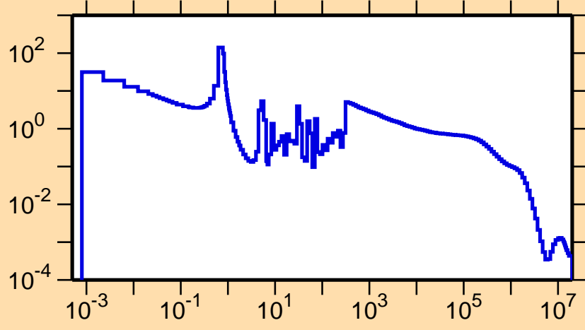
\sigma vs. E for ^{234}\text{Ac}(n,\gamma)
