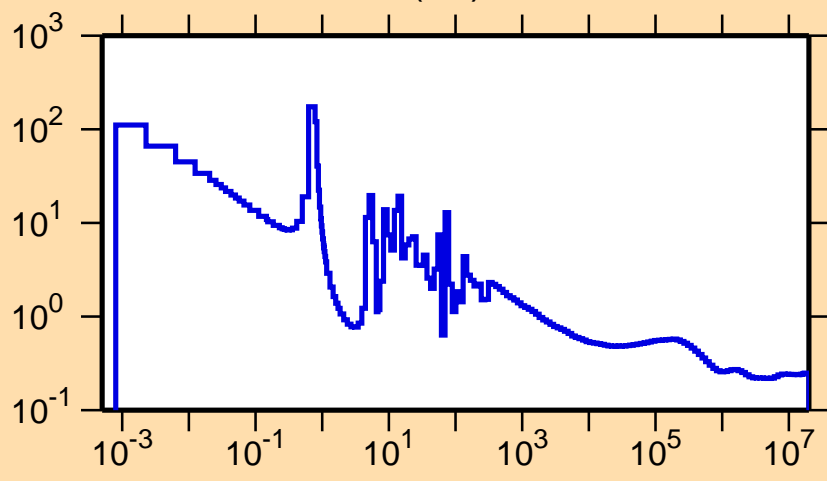
\sigma vs. E for ^{234}\text{Ac}(n,f)
