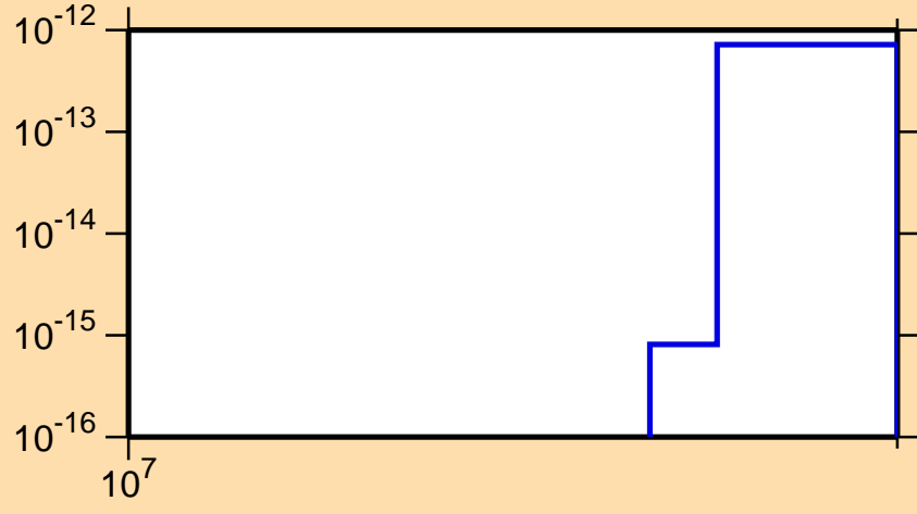
\sigma vs. E for ^{234}\text{Ac}(\text{mt } 11)
