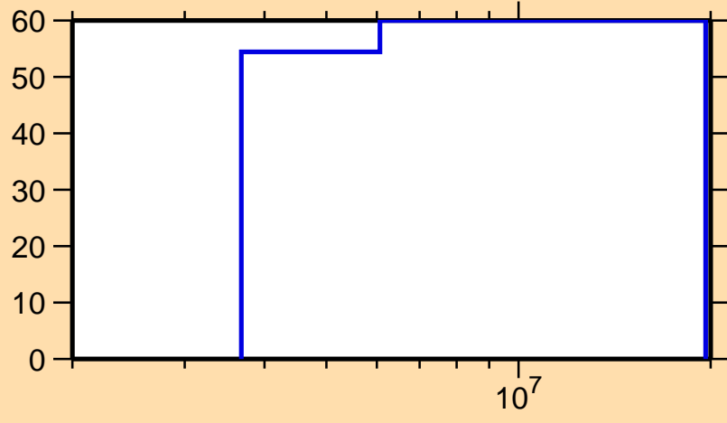
\Delta\sigma/\sigma vs. E for ^{234}\text{Ac}(n,p)
