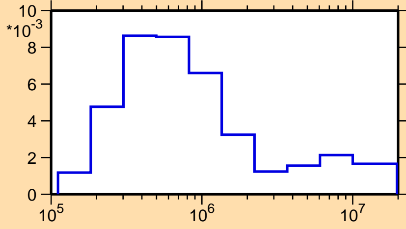
\sigma vs. E for ^{234}\text{Ac}(n,n_1)
