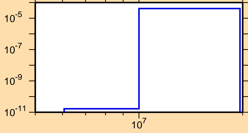
\sigma vs. E for ^{234}\text{Ac}(n,t)
