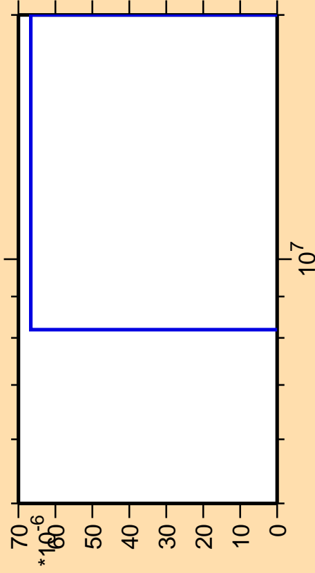
\Delta\sigma/\sigma vs. E for ^{234}\text{Ac}(n,\text{He3})
