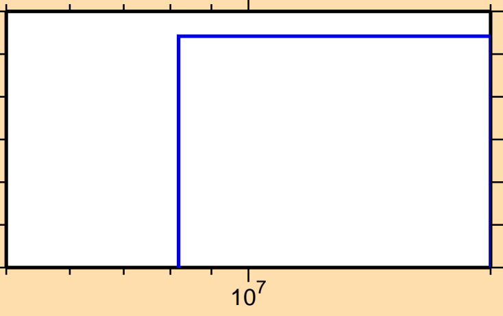
\sigma vs. E for ^{234}\text{Ac}(n,np)
