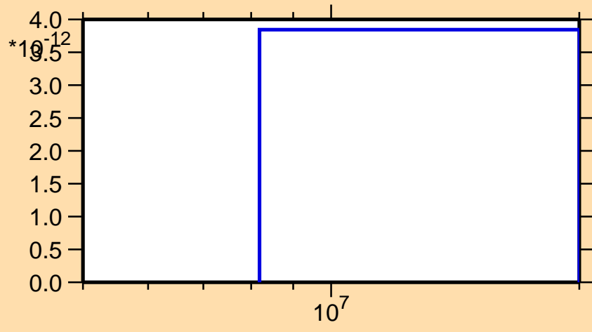
\sigma vs. E for ^{234}\text{Ac}(n,3n\alpha)
