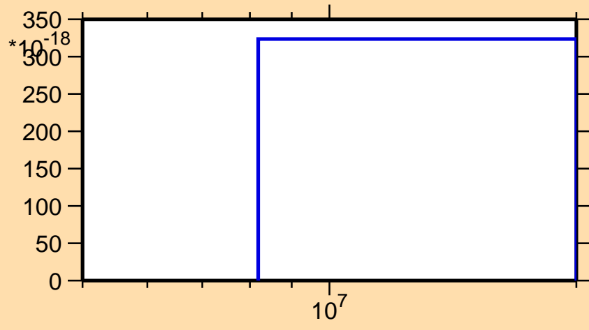
\sigma vs. E for ^{234}\text{Ac}(n,\text{He3})
