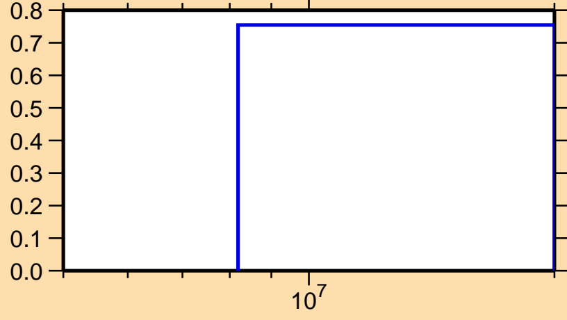
\sigma vs. E for ^{234}\text{Ac}(n,3n)
