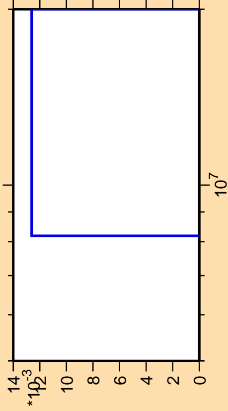
\Delta\sigma/\sigma vs. E for ^{234}\text{Ac}(\text{mt } 11)
