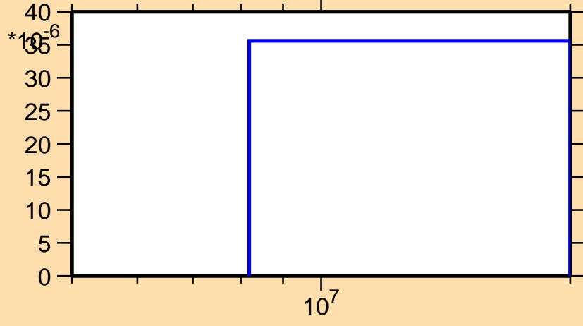
\sigma vs. E for ^{234}\text{Ac}(n,d)
