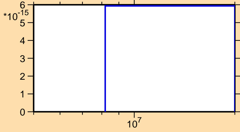
\sigma vs. E for ^{234}\text{Ac}(\text{mt } 11)
