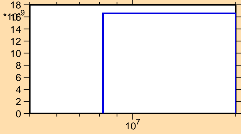
\sigma vs. E for ^{234}\text{Ac}(n,2np)
