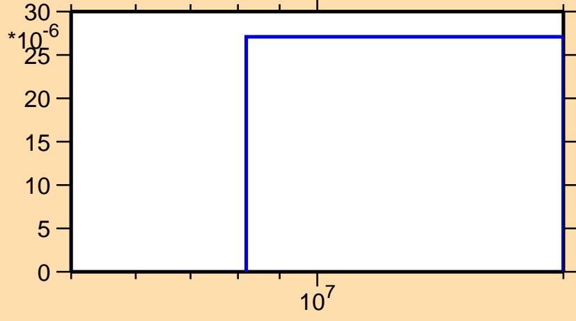
\sigma vs. E for ^{234}\text{Ac}(n,np)
