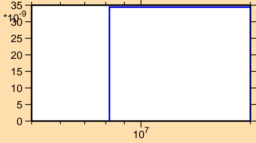
\sigma vs. E for ^{234}\text{Ac}(n,2n\alpha)
