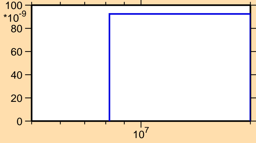
\sigma vs. E for ^{234}\text{Ac}(n,nt)
