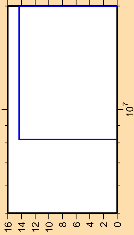
\Delta\sigma/\sigma vs. E for ^{234}\text{Ac}(n,3n\alpha)
