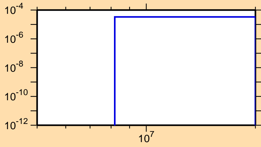
\sigma vs. E for ^{234}\text{Ac}(n,t)
