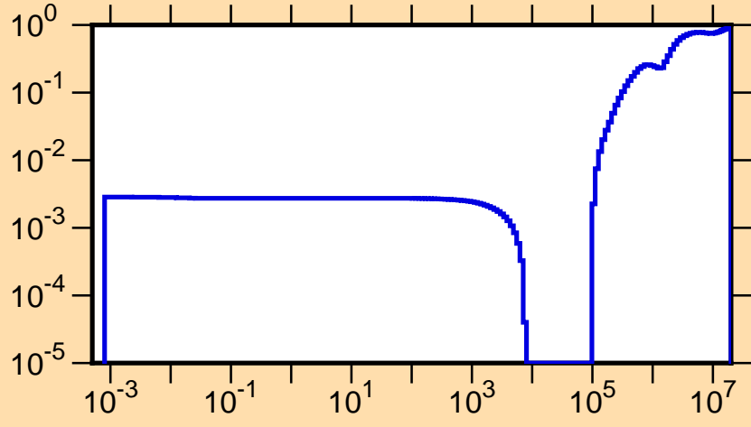
\mu vs. E for ^{235}\text{Ac}(\text{mt251})
