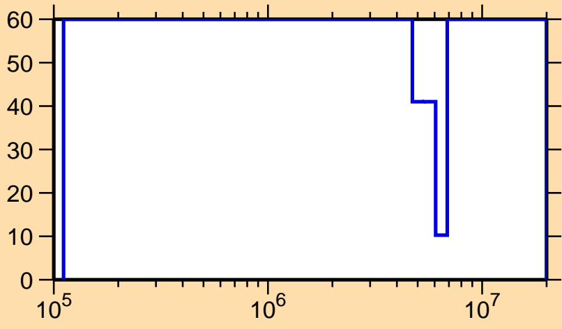
\Delta\sigma/\sigma vs. E for ^{235}\text{Ac}(n,n_1)
