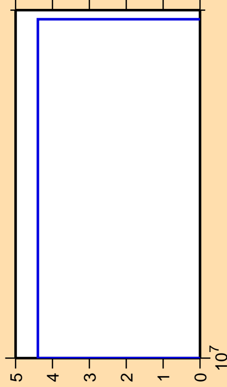
\Delta\sigma/\sigma vs. E for ^{235}\text{Ac}(n,3n\alpha)
