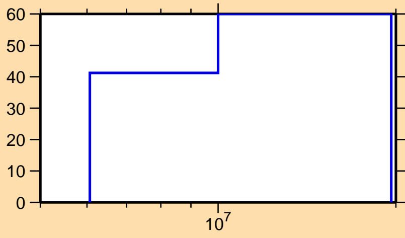
\Delta\sigma/\sigma vs. E for ^{235}\text{Ac}(n,n\text{cont.})
