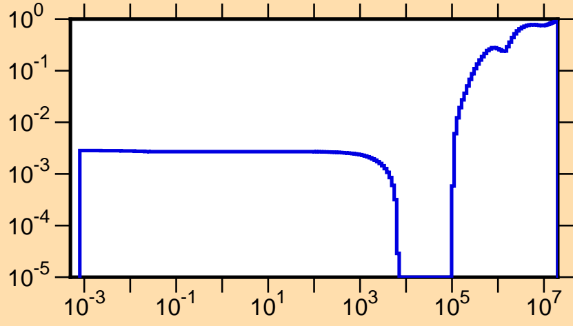
\mu vs. E for ^{236}\text{Ac}(\text{mt251})
