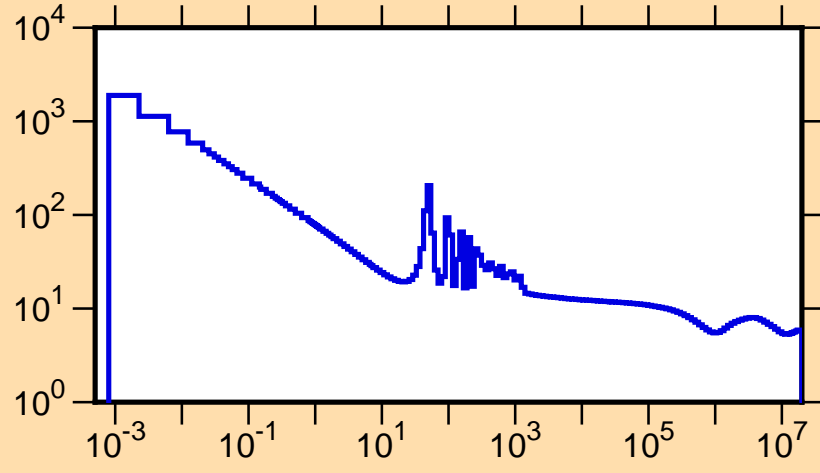
\sigma vs. E for ^{236}\text{Ac}(n,\text{tot.})
