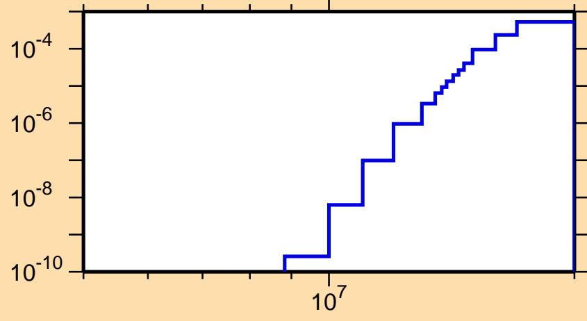
\sigma vs. E for ^{236}\text{Ac}(n,t)
