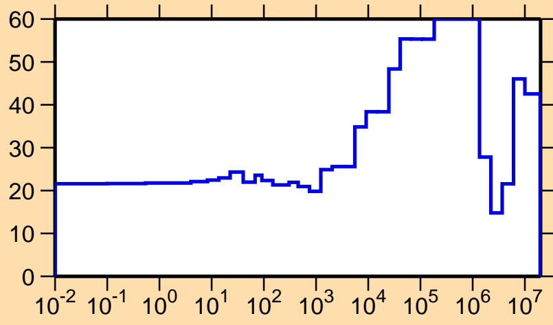
\Delta\sigma/\sigma vs. E for ^{236}\text{Ac}(n,el.)
