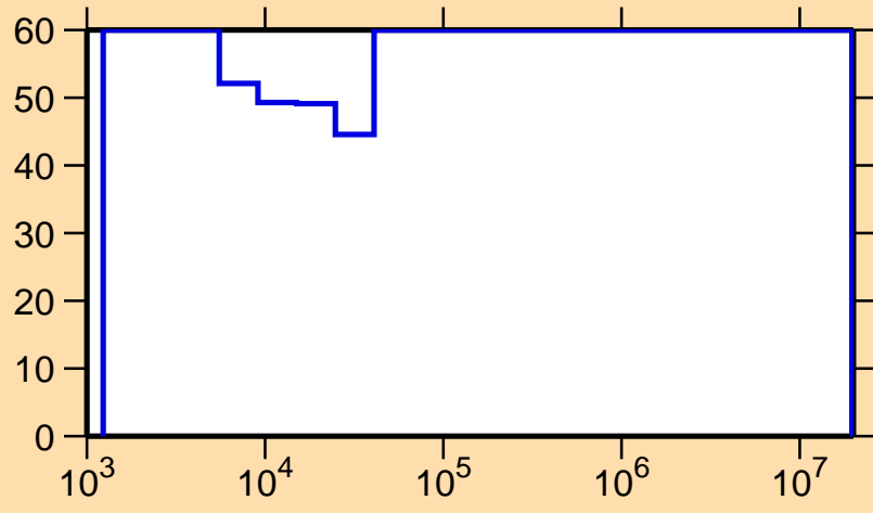
\Delta\sigma/\sigma vs. E for ^{236}\text{Ac}(n,\gamma)
