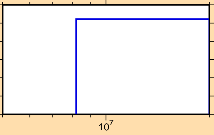
\sigma vs. E for ^{236}\text{Ac}(n,nt)
