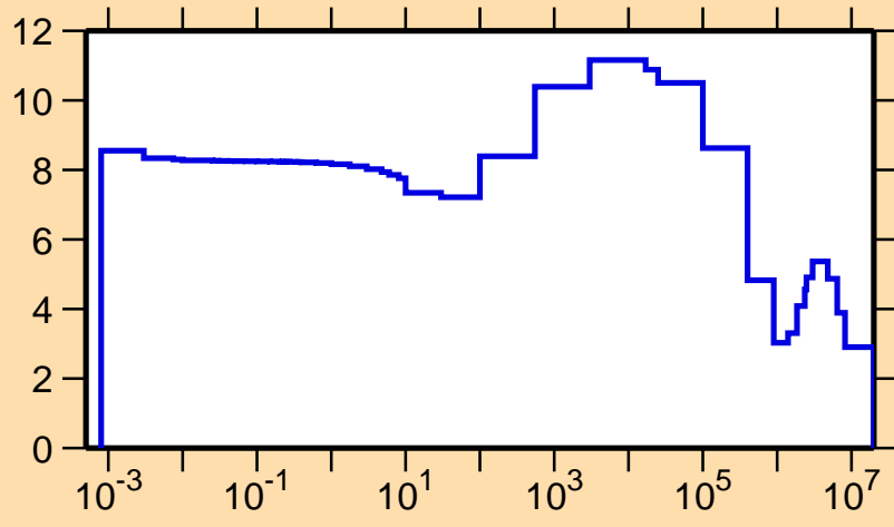
\sigma vs. E for ^{236}\text{Ac}(n,\text{el.})
