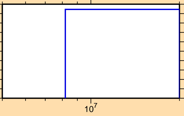
\sigma vs. E for ^{236}\text{Ac}(n,2n\alpha)
