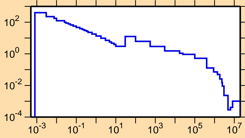
\sigma vs. E for ^{236}\text{Ac}(n,\gamma)
