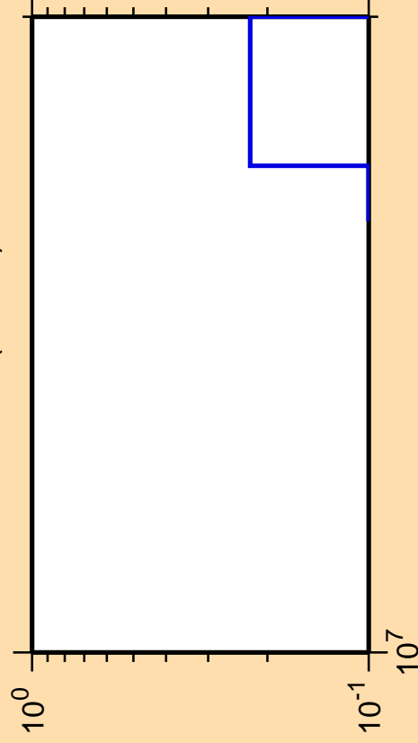
\Delta\sigma/\sigma vs. E for ^{237}\text{Ac} (mt 42)
