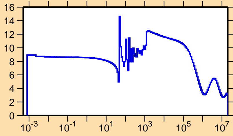
\sigma vs. E for ^{237}\text{Ac}(n,\text{el.})
