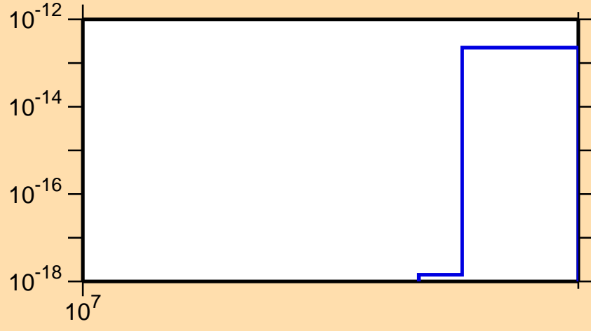
\sigma vs. E for ^{237}\text{Ac} (mt 42)
