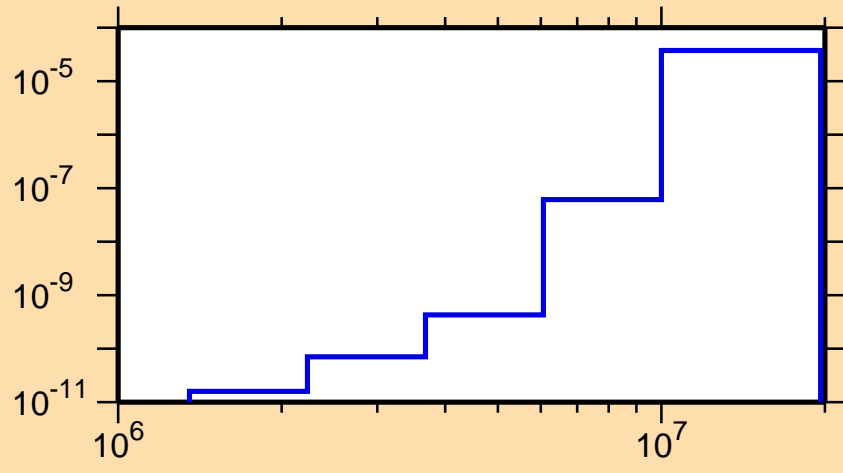
\sigma vs. E for ^{237}\text{Ac}(n,\alpha)
