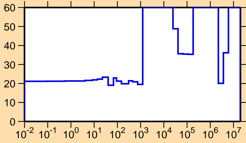
\Delta\sigma/\sigma vs. E for ^{237}\text{Ac}(n,el.)
