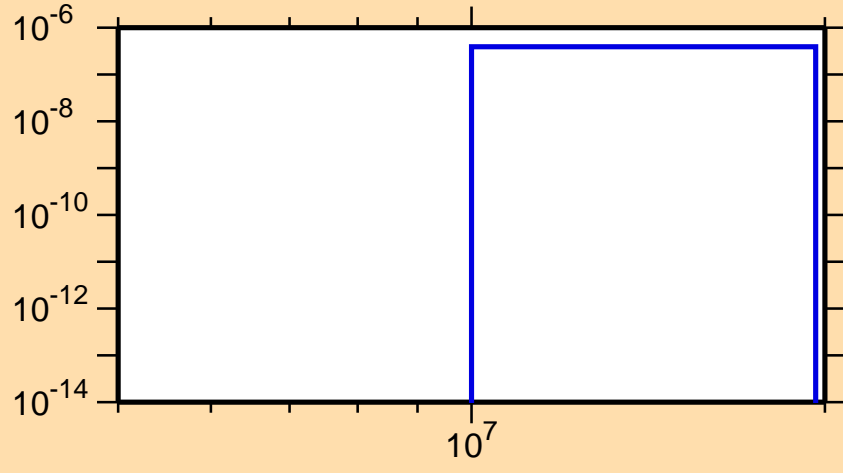
\sigma vs. E for ^{237}\text{Ac}(n,nt)
