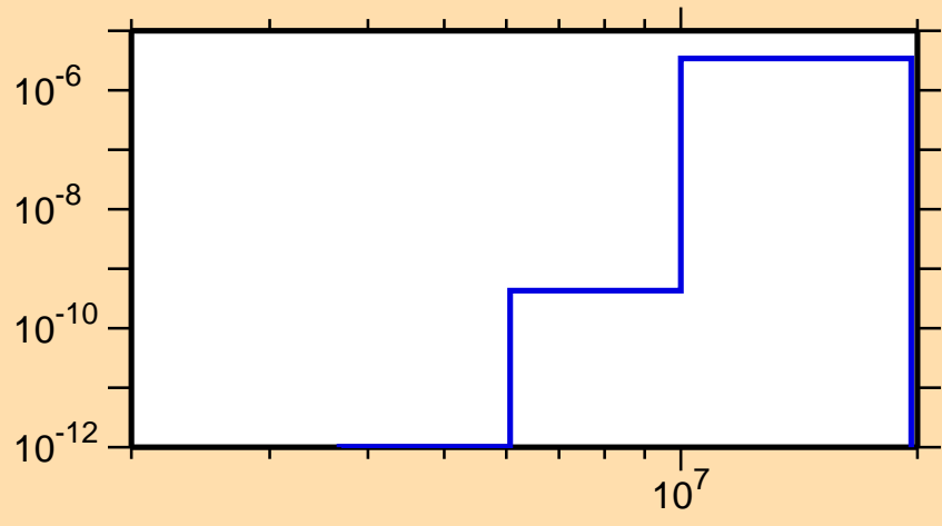
\sigma vs. E for ^{237}\text{Ac}(n,n\alpha)
