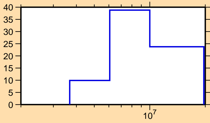
\Delta\sigma/\sigma vs. E for ^{237}\text{Ac}(n,\text{tot.})
