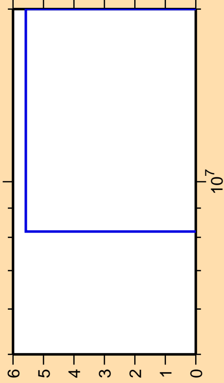
\Delta\sigma/\sigma vs. E for ^{237}\text{Ac}(n,3n\alpha)
