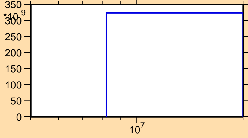
\sigma vs. E for ^{237}\text{Ac}(n,nt)
