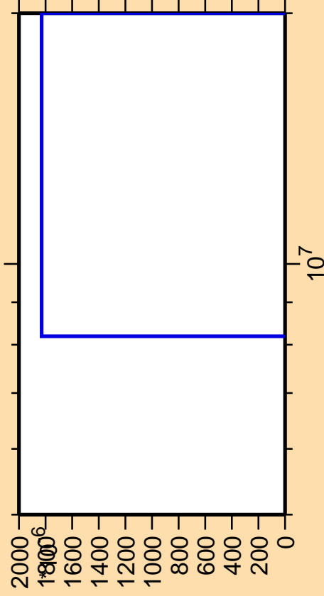
\Delta\sigma/\sigma vs. E for ^{237}\text{Ac} (mt 42)
