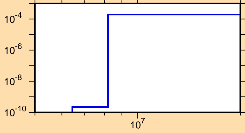
\sigma vs. E for ^{237}\text{Ac}(n,p)
