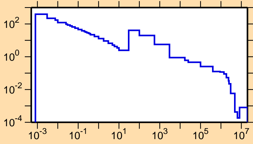
\sigma vs. E for ^{237}\text{Ac}(n,\gamma)
