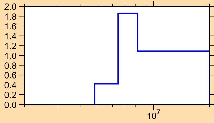
\sigma vs. E for ^{237}\text{Ac}(n,2n)
