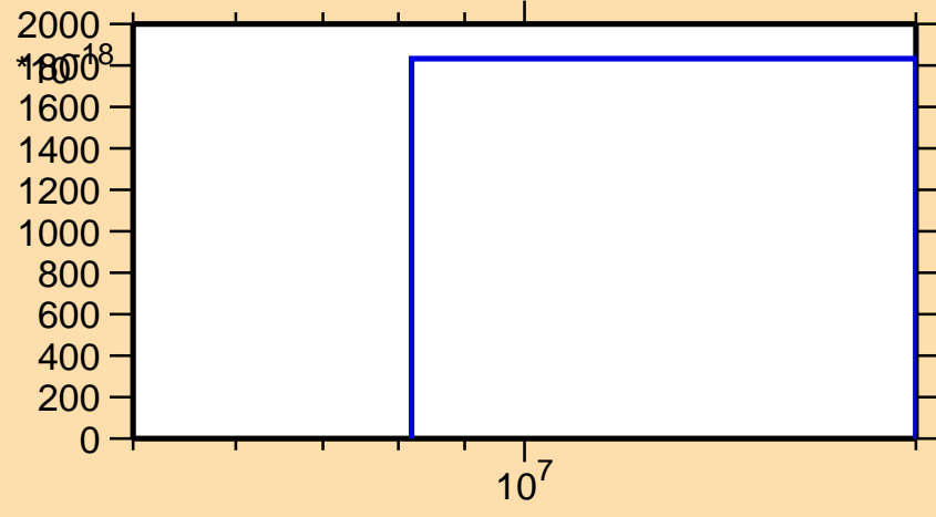
\sigma vs. E for ^{237}\text{Ac} (mt 42)
