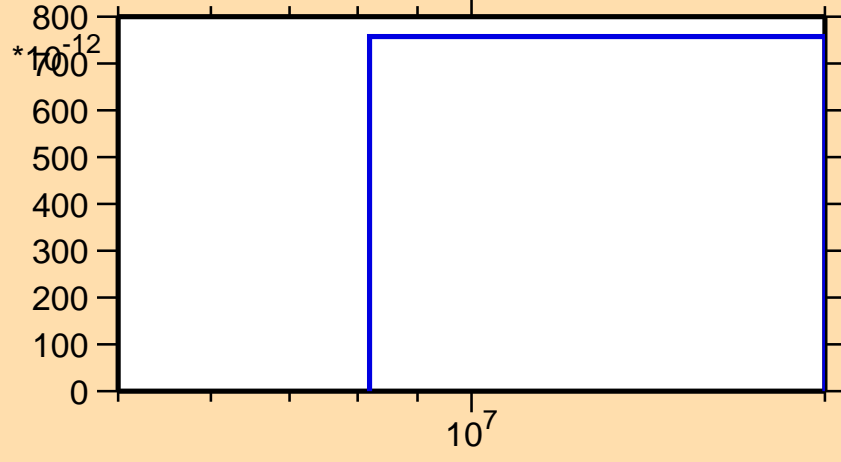
\sigma vs. E for ^{237}\text{Ac}(n,2np)
