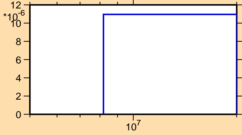
\sigma vs. E for ^{237}\text{Ac}(n,np)
