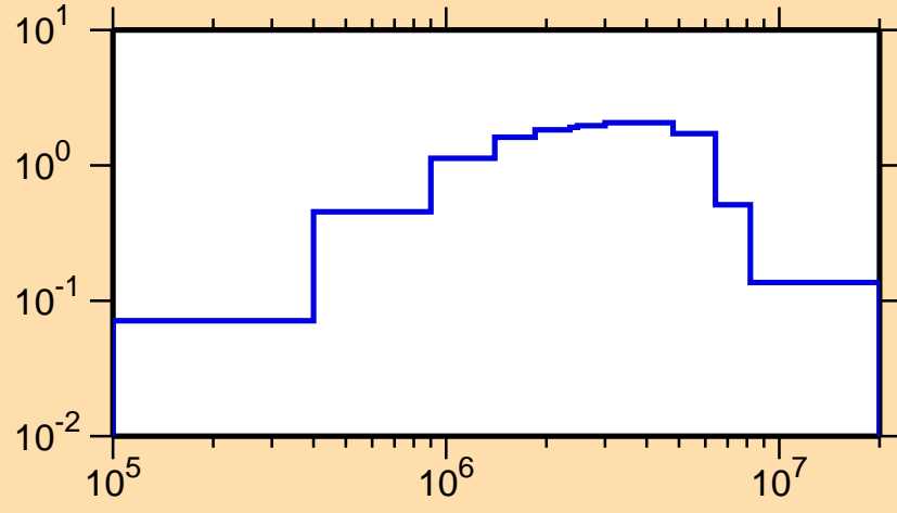
\sigma vs. E for ^{237}\text{Ac}(n,n\text{cont.})
