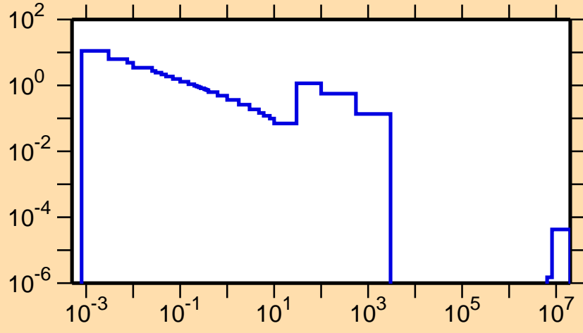
\sigma vs. E for ^{237}\text{Ac}(n,f)
