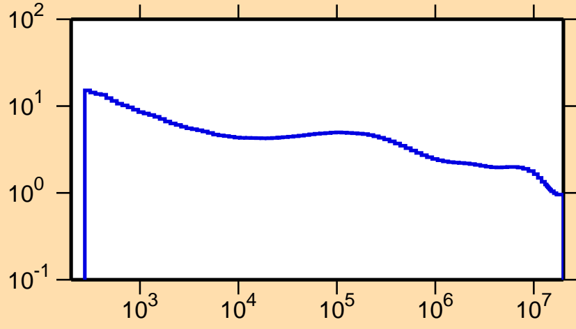
\sigma vs. E for ^{95}\text{Ag}(n,\text{nonel.})
